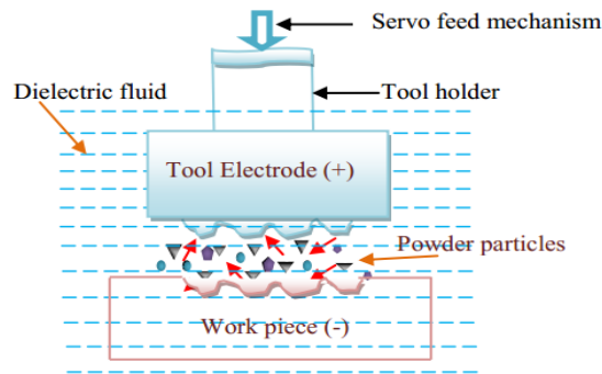
Figure (1) the principle of PMEDM [5]
