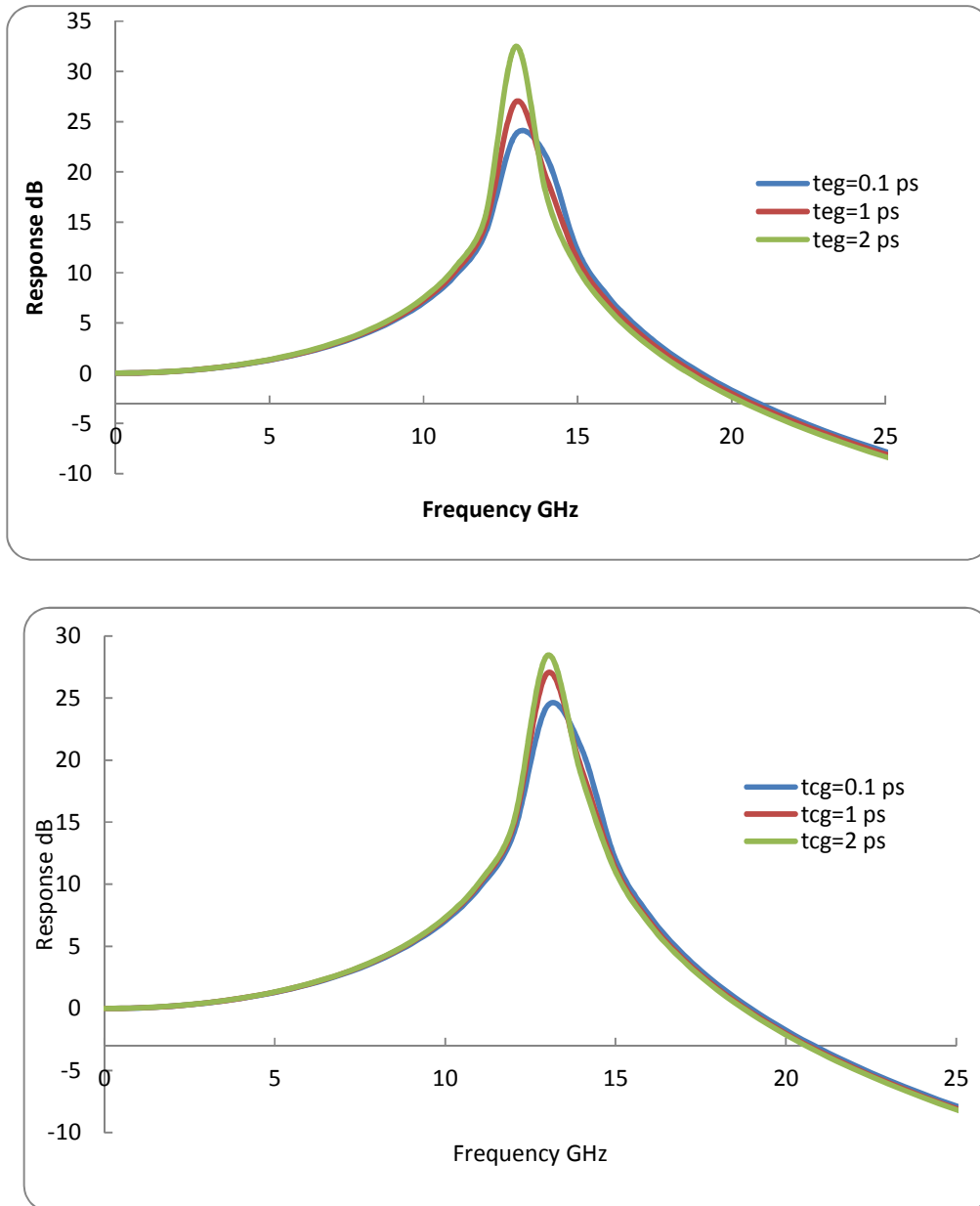
Figure (6) Effect of \tau_{ce} and \tau_{eg} on the small signal modulation response.
