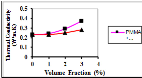
Figure 4: Shows thermal conductivity of PMMA composite materials as function of (Nano-SiO 2 - Nano-Al 2 O 3 ) particles (Vol %) in composite
