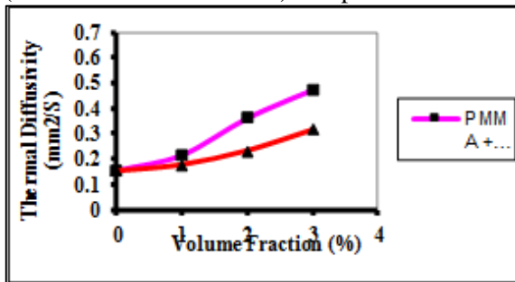
Figure 5: Shows thermal diffusivity of PMMA composite materials as function of (Nano-SiO 2 - Nano-Al 2 O 3 ) particles (Vol %) in Co
