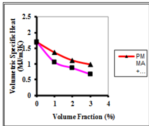
Figure 6: Shows volumetric specific heat of PMMA composite materials as function of (nano-SiO 2 - nano-Al 2 O 3 ) particles (Vol %) in composite.
