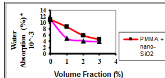
Figure 3: Shows Water Absorption Percentage of PMMA Composite Materials as Function of (Nano- \text{SiO}_2 - Nano- \text{Al}_2\text{O}_3 ) Particles (Vol %) in Composite
