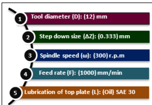
Figure 6: The proposed parameters constant
