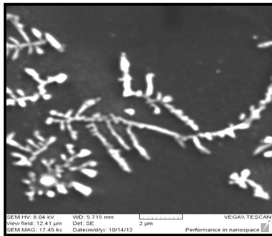
Figure 3: SEM micrographs of the prepared AgNPs using first method (AgNPs) at T=100^{\circ}\text{C}
