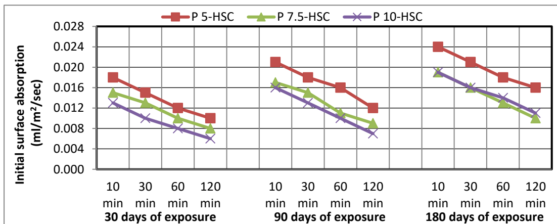
Fig. 11. Initial surface absorption of LM-HSC exposed to gasoline and coated by epoxy.
