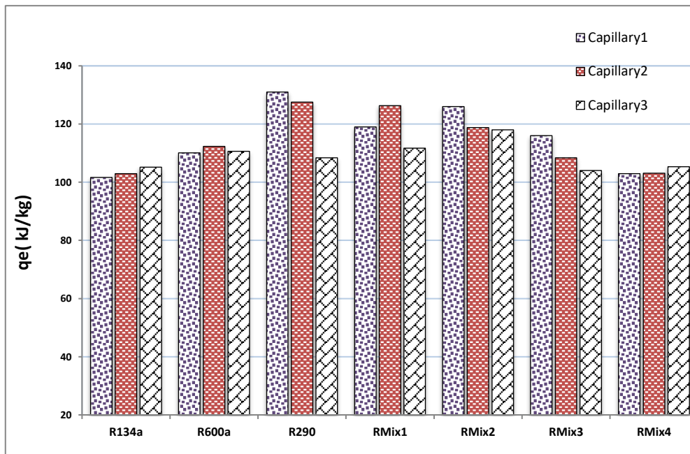
Fig. 6. Refrigerating capacity Vs capillary tube diameter.
