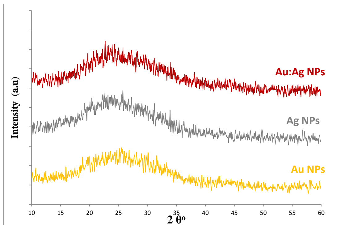
Figure 3: XRD pattern of Au, Ag and Au:Ag NPs.
