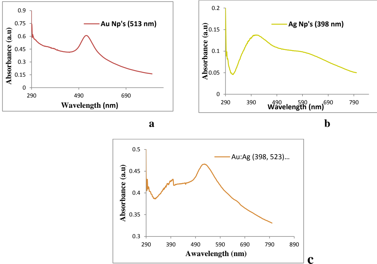
Figure 1: Optical Absorbance spectra (SPR band) of a. Au, b. Ag and c. Au:Ag NPs.
