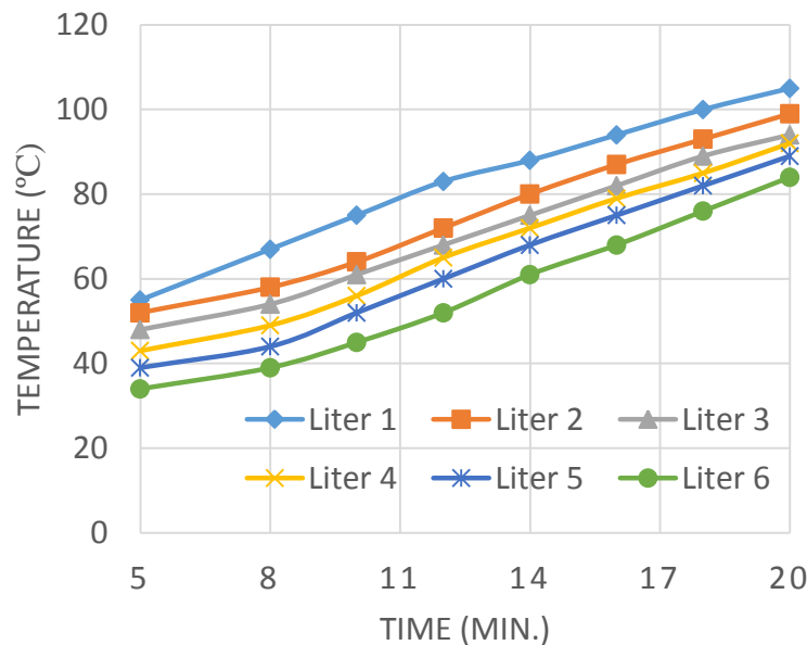
Fig. 2: The relation between the temperature of cooking fluid and time of trial at different amounts of water.
