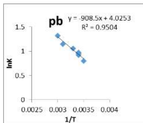
Figure(10)Vant Huff curve of (Pb)
