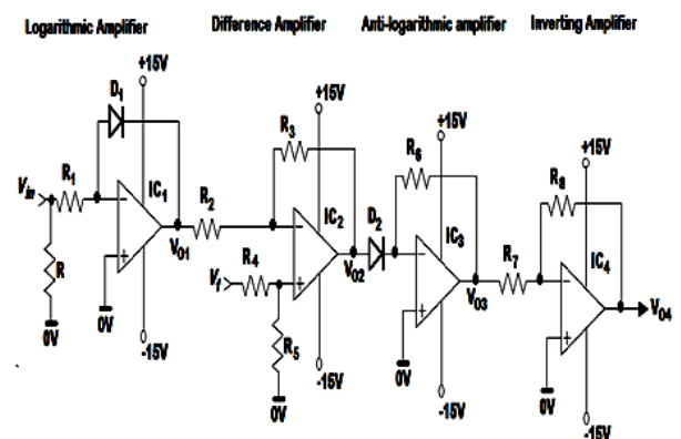
Figure 3: Circuit diagram of the proposed system
