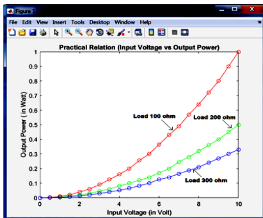
Figure 6: Practical relation between consumed power and applied voltage using the proposed circuit
