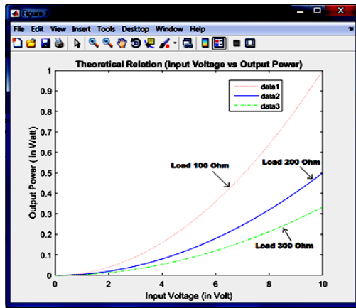
Figure 5: Theoretical relation between consumed power and applied voltage using the proposed circuit
