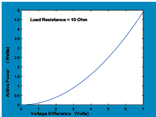
Figure 8: The result of relation between the actual power and the applied voltage of the work of Ilsche et al. [9]
