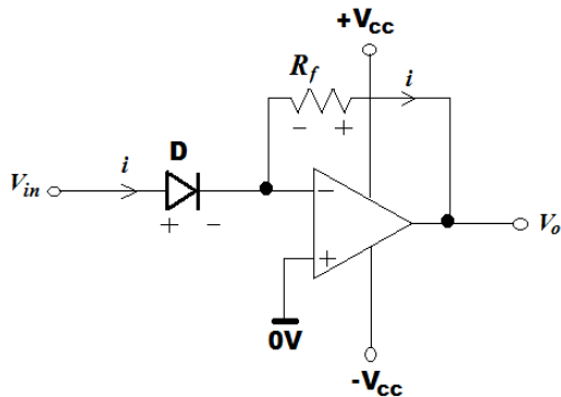
Figure 2: Circuit diagram of the anti-logarithmic amplifier
