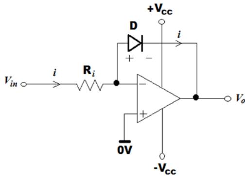
Figure1: Circuit diagram of the logarithmic amplifier
