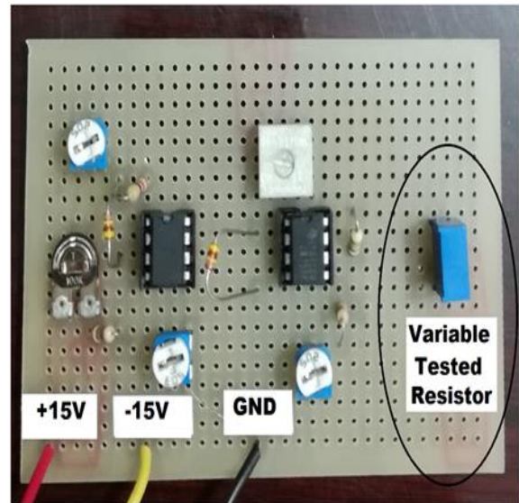
Figure 4: Implementation of the proposed circuit on printed circuit board (PCB)
