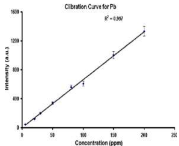
Figure 1: Standard calibration curve of lead
