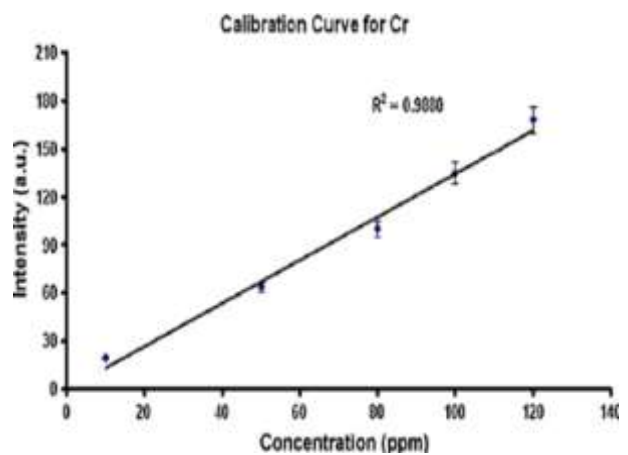
Figure 2: Standard calibration curve of chromium
