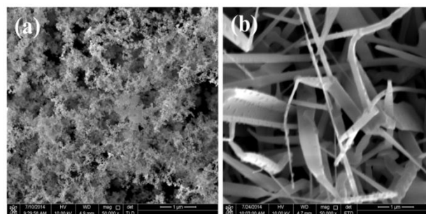
Figure 1: FESEM image of the catalyst-free growth of 2D and 3D ZnO nanostructures on ZnO seed layer under different Ar flow rates (a) 10 ml/min, and (b) 40 ml/min.
