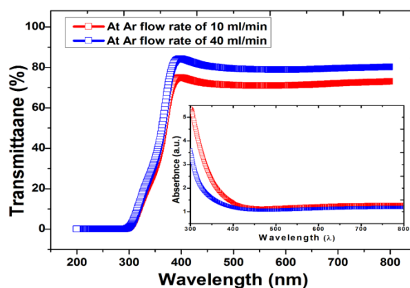
Figure 3: UV–Vis transmissions of the 2D and 3D ZnO nanostructures under different Ar flow rates. The absorption spectrum is shown in the inset.
