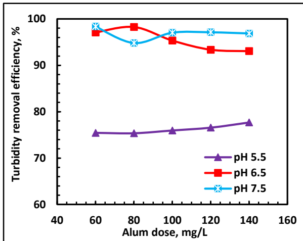
Fig. 4. Effect of alum dose on turbidity removal efficiency at different pH, Nickel dose 240 mg/L
