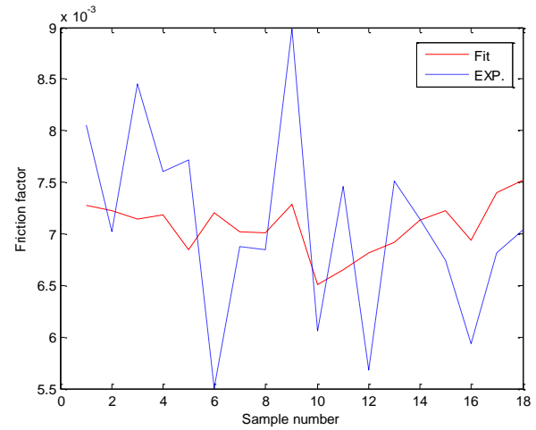
Fig. 21. Comparison of friction factor (correlation vs. experimental results).
