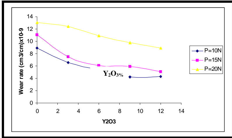
Figure (10) showing the relationship between the \text{Y}_2\text{O}_3\% and wear rate at the 30 min time test.
