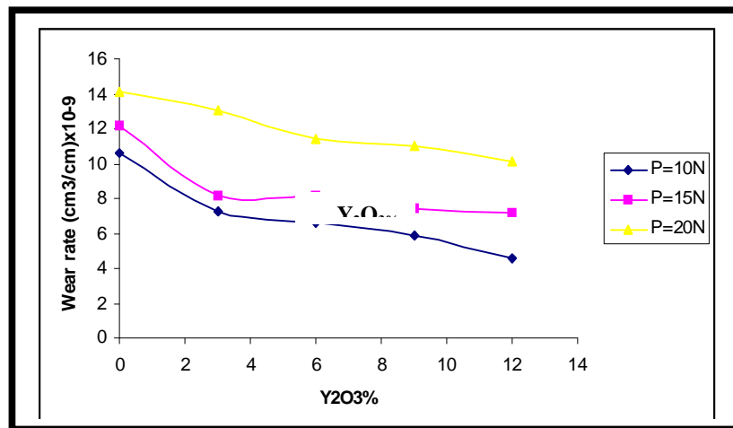
Figure (11) showing the relationship between the \text{Y}_2\text{O}_3\% and wear rate at the 45 min time test.
