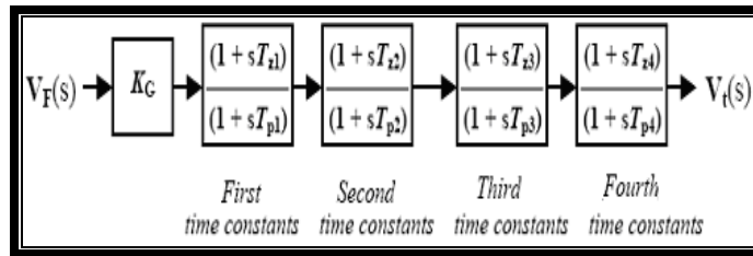
Figure (3) Block diagram representing a 4th order SG time constants model
