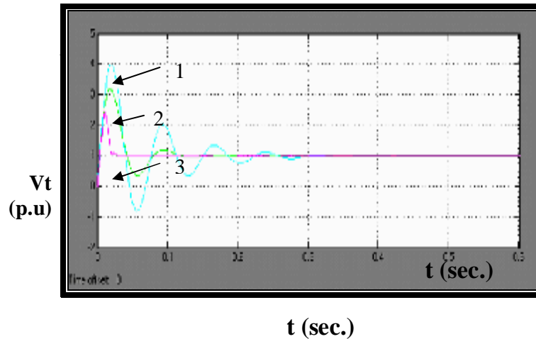
Figure (17) V_t transient responses of the 4th order SG model for 0.6 p.u. load change with different types of controllers
