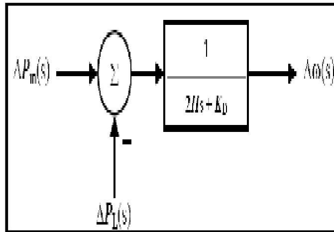
Figure (1) Block diagram of a load change model.
