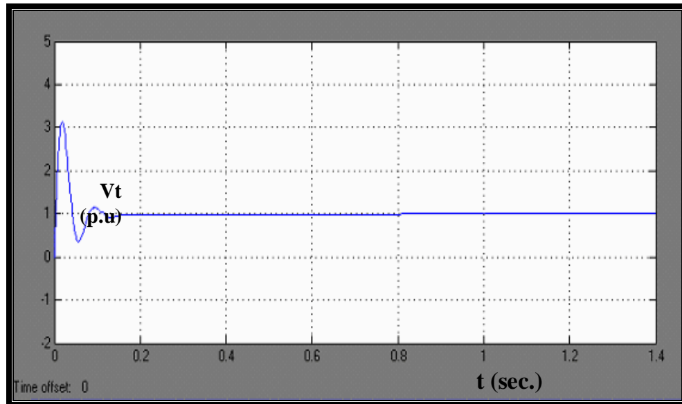
Figure (12) Terminal voltage when K_p = 1, K_i = 0.5, \text{ and } K_d = 0.005
