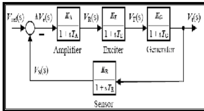
Figure (4) Block diagram of a simple AVR [11]
