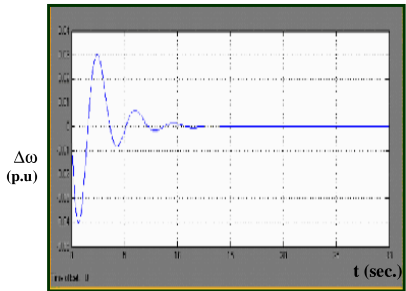
Figure (10) Frequency deviation ( \Delta\omega ) for 0.6p.u load change
