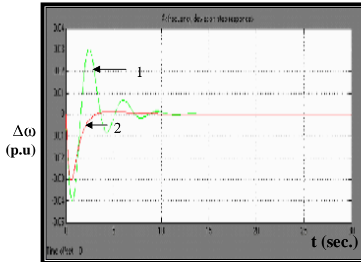
Figure (18) Freq. Deviation ( \Delta\omega ) step responses of the 4th order SG model for 0.6 p.u. load change .
