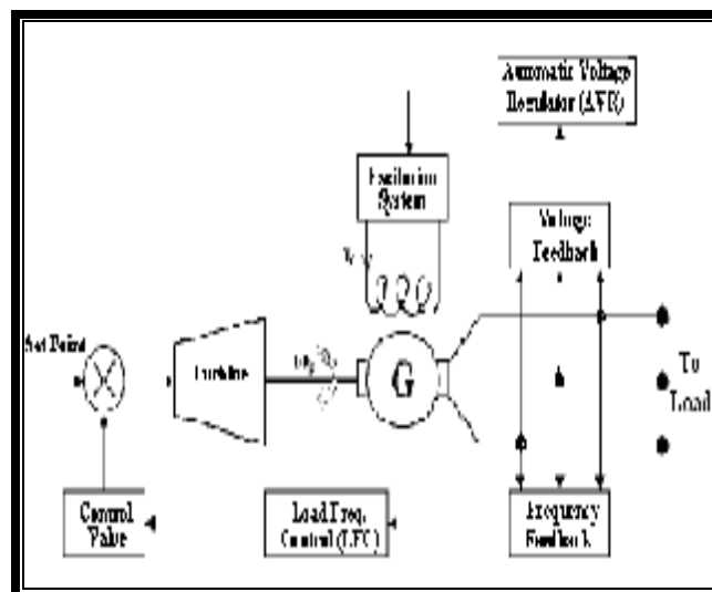
Figure (2) Block Diagram of Governor and AVR of the SG [7].
