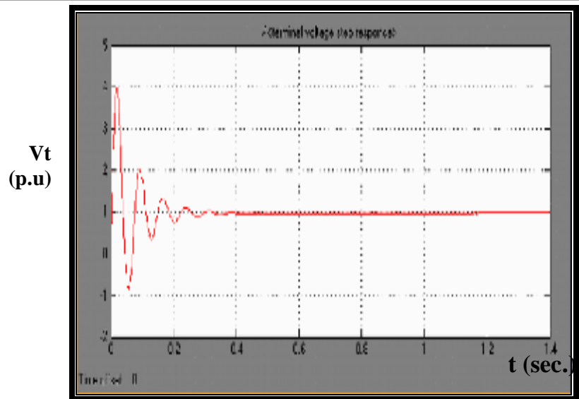
Figure (9) Terminal voltage ( V_t ) step response for 0.6p.u load change
