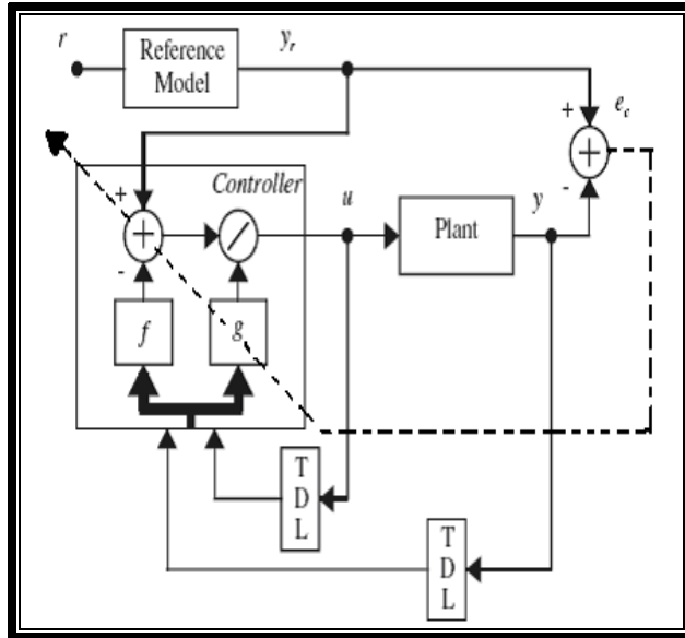
Figure (7) The block diagram of NARMA-L2 with the reference model and plant
