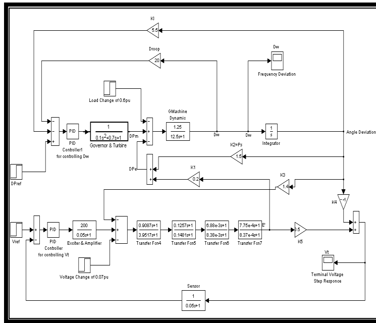
Figure (11) Simulation Model for the 4th Order SG with PID Controller
