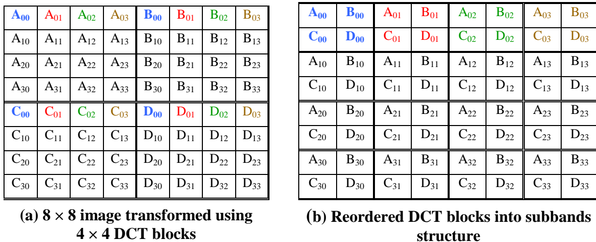
Figure (2): The two different representations of DCT coefficients. (a) The block representation and (b) The subband representation
