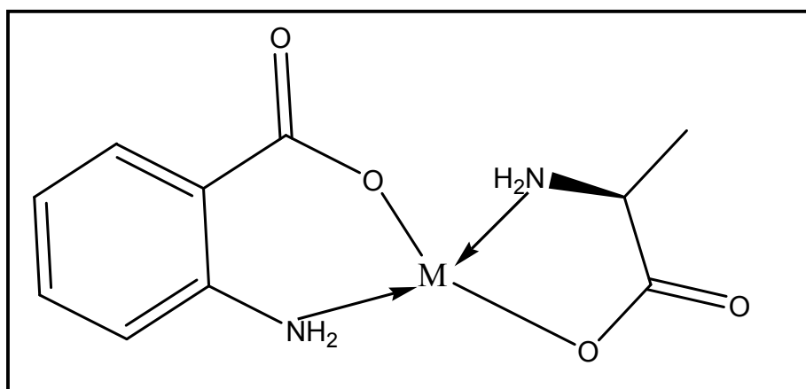
Fig (1) : The proposed structure of the complexes [M(\text{A})(\text{Ala})] .
