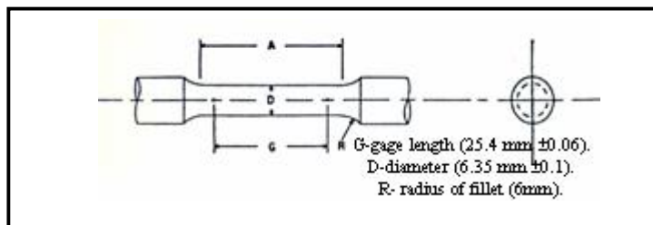
Fig. (3) The dimensions of the tensile.
