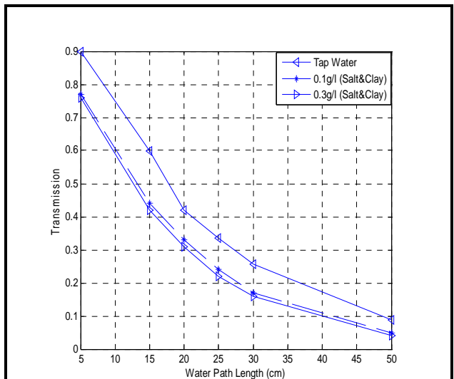
Fig. 5 the variety of laser transmission against the water path length.
