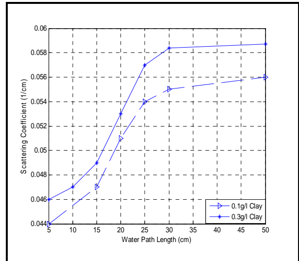
Fig. 8 the variety of scattering coefficient against water path length of distill water contained 0.1g/l and 0.3g/l of clay
