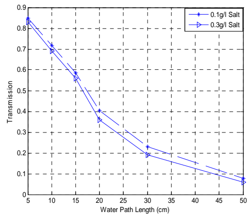
Fig. 7 the variety of laser transmission against water path length of distill water contained 0.1g/l and 0.3g/l of salt.
