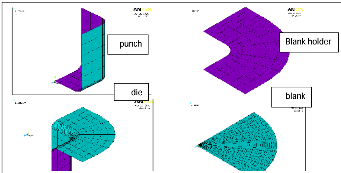
Figure (1) Finite element model of the sheet material and drawing die.
