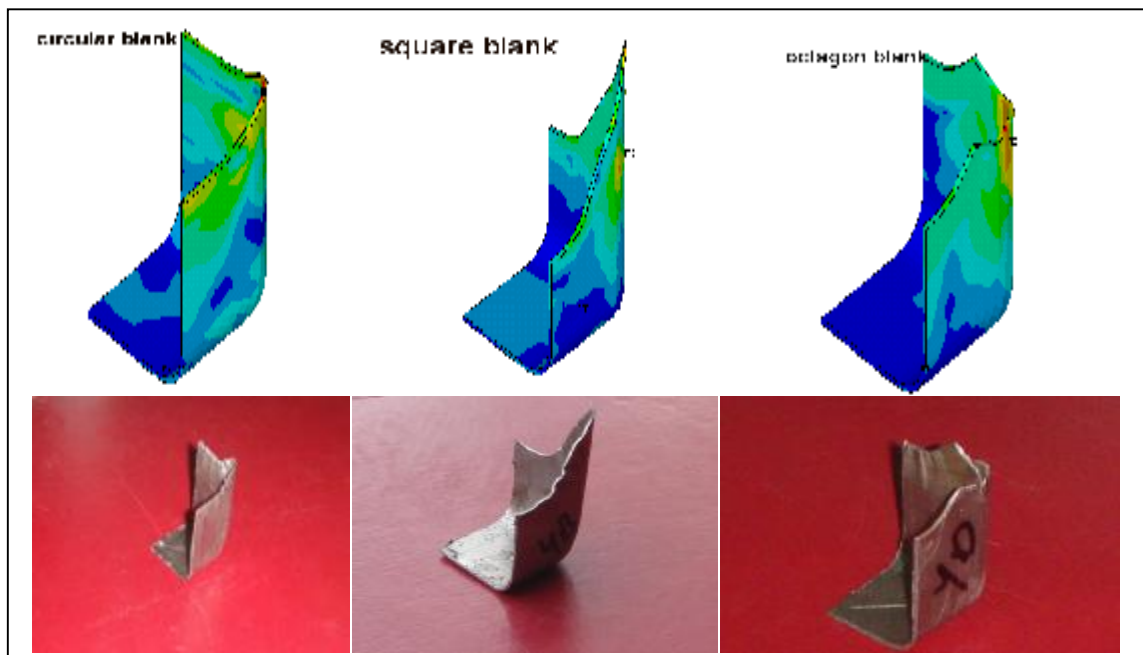
Figure (5) Comparison of cup shape (earing shape) between FEM model and experimental work. (rd5,rp5, \mu 0.1 ,v60,bhf15).
