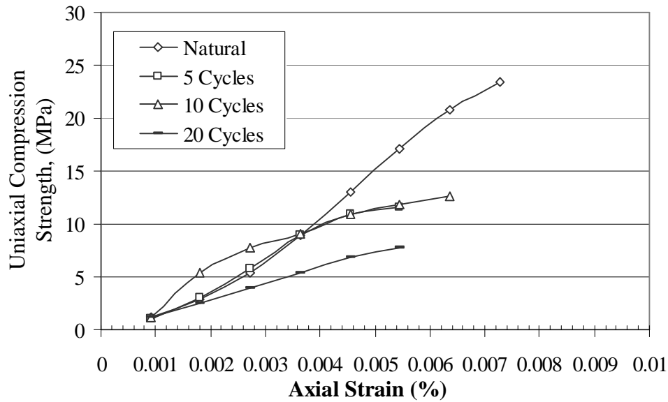
Figure (12) Effect of Freezing-Thawing Cycles on Stress-Strain Curves for Rock Type (L2)
