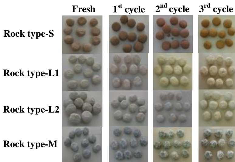
Figure (4) Changes in Shape of Specimens During Slaking Durability Test
