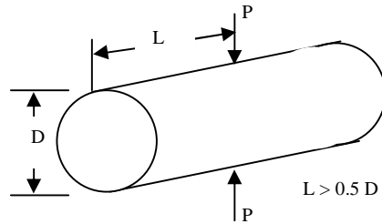
Figure (3), Specimen dimension in the point load test
