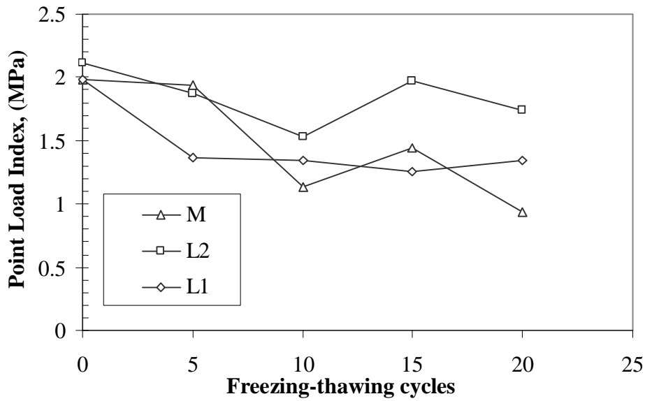
Figure (14) Effect of Freezing-Thawing Cycles on the Point Load Strength Index of the Studied Rock
