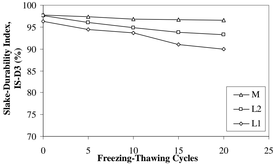
Figure (6) Effect of Freezing-Thawing Cycles on the Slake-Durability Index of the Studied Rocks
