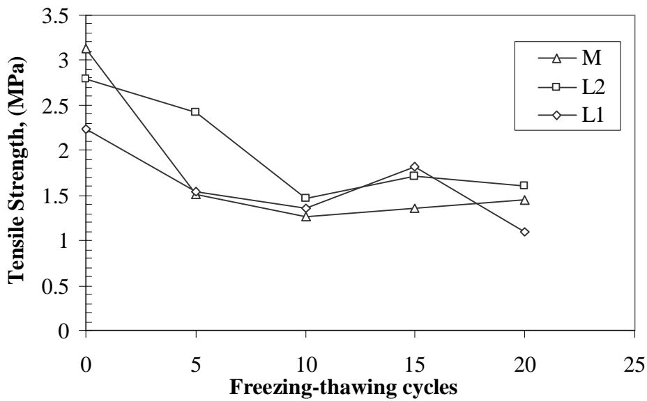
Figure (15) Effect of Freezing-Thawing Cycles on the Tensile Strength of the Studied Rocks
