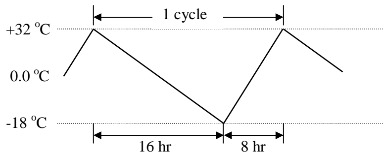
Figure (2) Schematic sketch of 1 cycle freeze-thaw test
