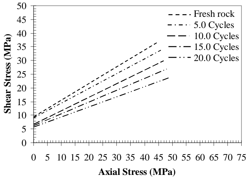
Figure (9) Mohre Envelope for Rock Type (M) from Triaxial Test at Various Freezing-Thawing Cycles
