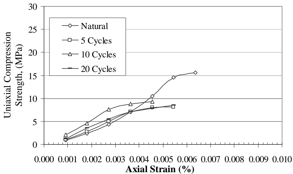
Figure (11) Effect of Freezing-Thawing Cycles on Stress-Strain Curves for Rock Type (L1)
