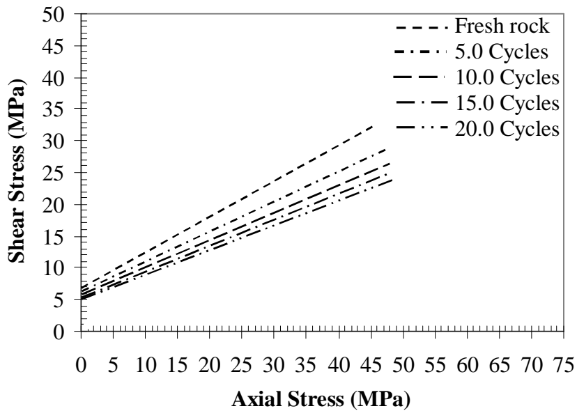
Figure (7) Mohre Envelope for Rock Type (L1) from Triaxial Test at Various Freezing-Thawing Cycles
