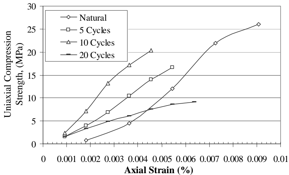
Figure (13) Effect of Freezing-Thawing Cycles on Stress-Strain Curves for Rock Type (M)
