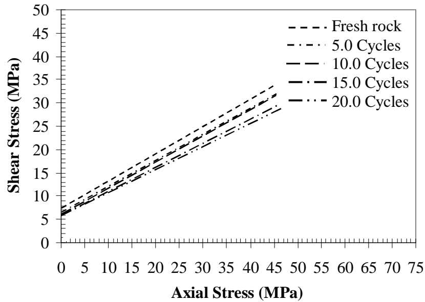
Figure (8) Mohre Envelope for Rock Type (L2) from Triaxial Test at Various Freezing-Thawing Cycles
