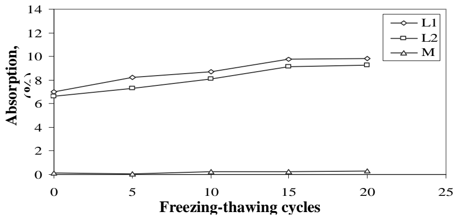
Figure (5) Effect of Freezing-Thawing Cycles on the Absorption Percent of the Studied Rocks
