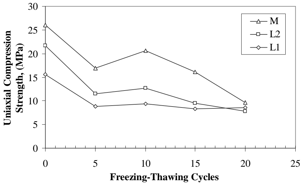
Figure (10) Effect of Freezing-Thawing Cycles on the Uniaxial Compression Strength of the Studies Rocks
