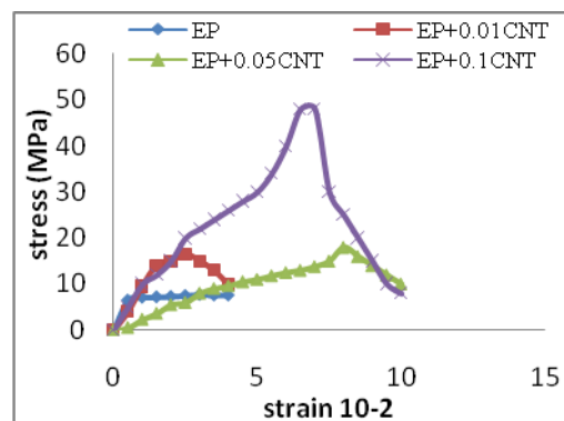
Fig: (2) Tensile stress –strain for epoxy composites
