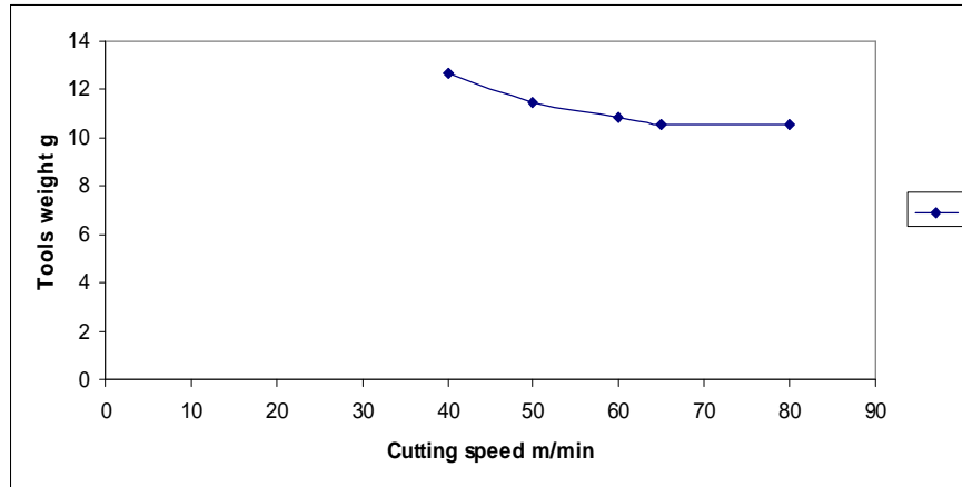
Figure (3) Relationship between cutting speed and weight of tool with B.U.E at 20% carbon
