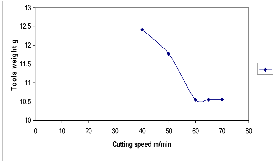
Figure ( 1 ) Relationship between cutting speed and weight of tool with B.U.E at 10% carbon
