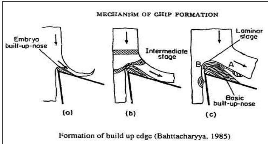
Figure ( 7 ) Mechanism of chip formation
