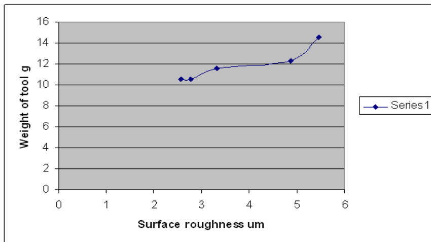
Figure (4) Relationship between surface roughness and weight of tool with B.U.E during machining workpiece 0.10% carbon
