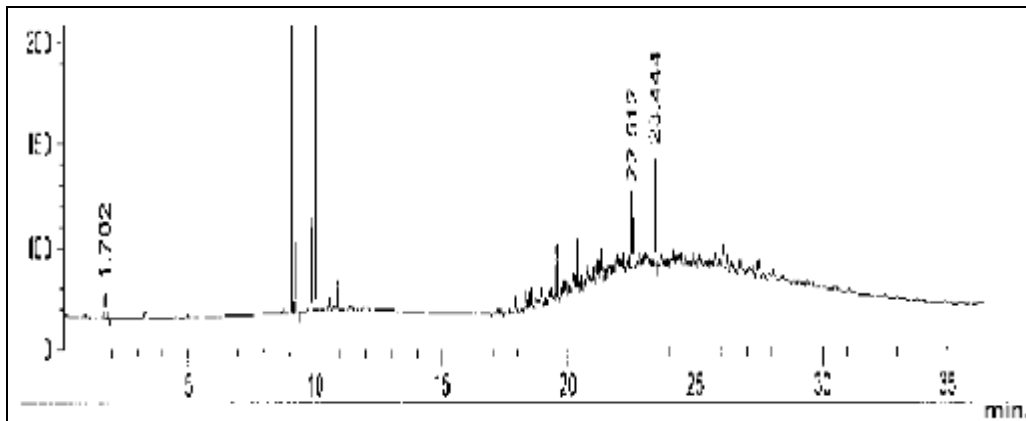
Figure (6) Gas Chromatogram of Hexane Extract of Surface in Dumping Lagoons
