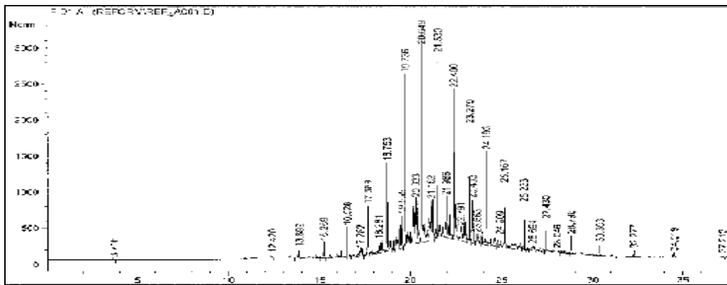
Figure (5) Gas Chromatogram of Dehydrated Gasoil
