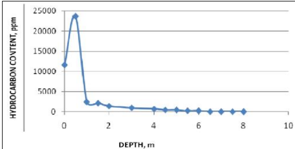
Figure (2) Distribution of Hydrocarbons with the Depth of Soil
