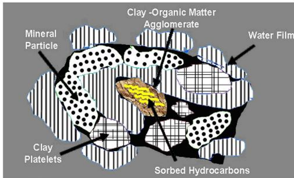
Figure (3) Hydrocarbon Interfractions with Soil [11].
