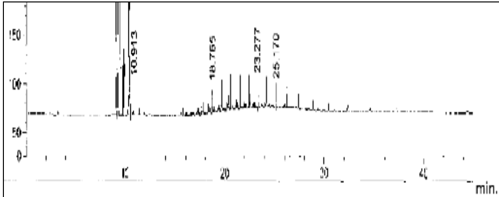
Figure (4) Gas Chromatogram of Hexane Extract of Soil at 100 cm Depth in Dumping Lagoons
