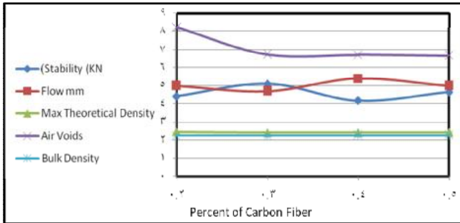
Figure (4) Marshall Properties of Stone Matrix Asphalt.
