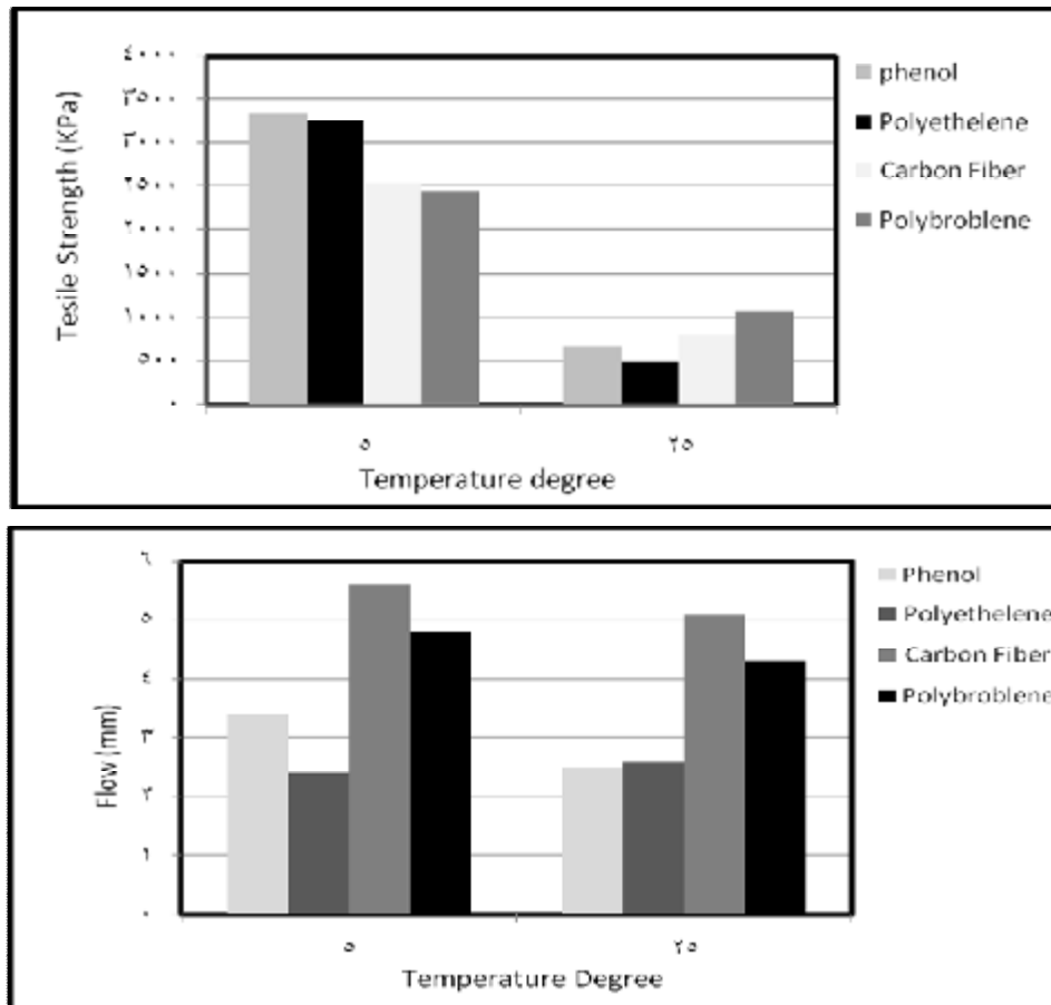
Figure (5) Tensile Strength and Flow value of Stone Matrix Asphalt.
