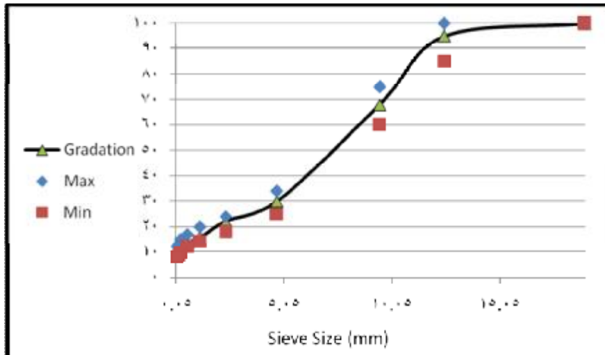
Figure (1) Selected Gradation of Aggregate.
