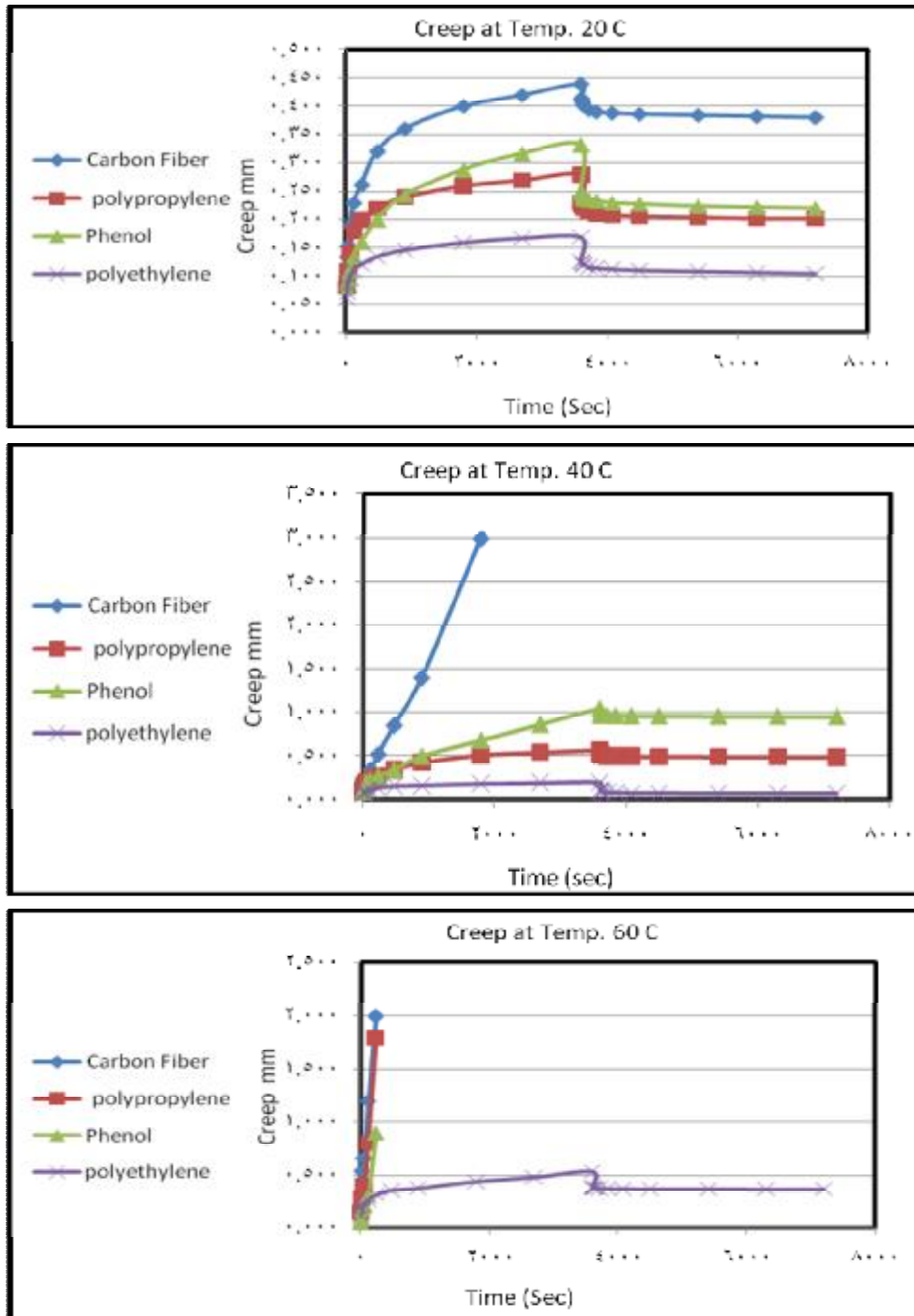
Figure (6) Creep Test at different Temperature 6426
