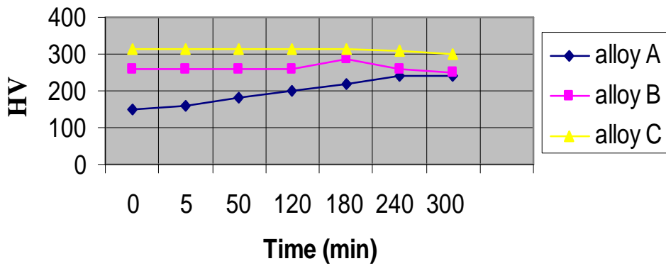
Figure (12 A) Precipitation hardening of Fe-Cu alloy after air cooling and aging at 480 o C
