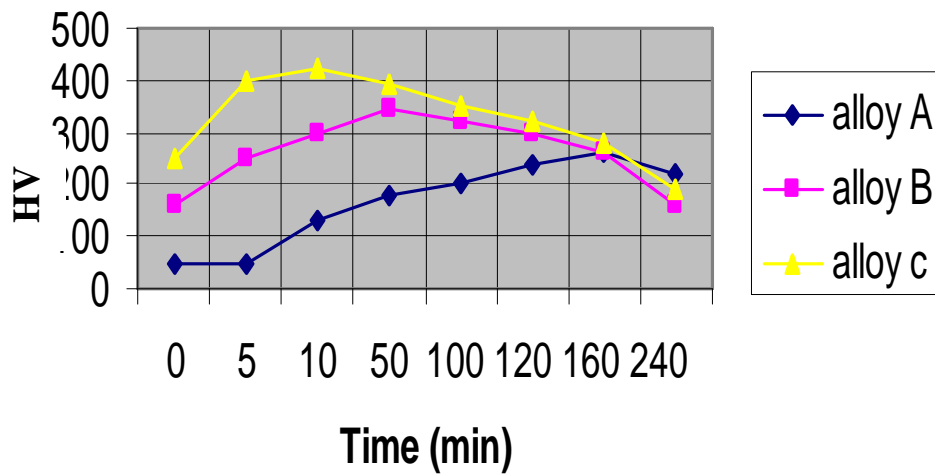
Figure (11 A) Precipitation hardening of Fe-Cu alloy after water quenching and aging at 480 °C
