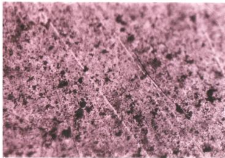
Figure (10) Microstructure of Fe-6% Cu-3%Ni alloys after air -cooled. ((Massive Martensite with precipitates of Cu and some particles of Fe 2 O 3 or Cu 2 O or Ni 2 O 3 )). (X200)
