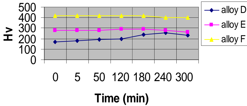
Figure (12 B) Precipitation hardening of Fe-Cu-Ni alloy after air cooling and aging at 480 o C
