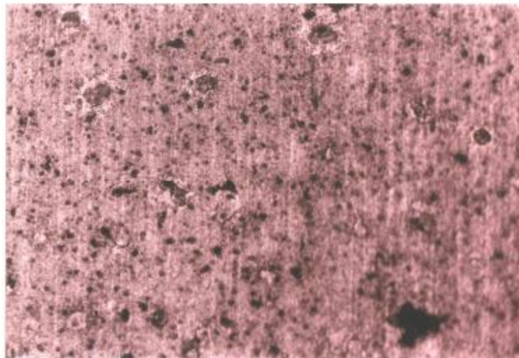
Figure (9) Microstructure of Fe-6% Cu alloys after air -cooled. (Massive Martensite with precipitates of Cu and some particles of Fe 2 O 3 orCu 2 O)). (X200)
