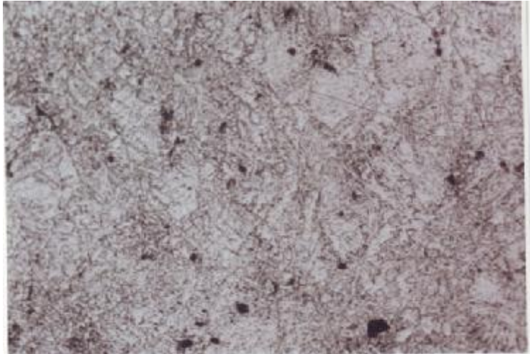
Figure (4) Microstructure of Fe-2% Cu-1%Ni alloys after air -cooled. (Massive Ferrite with precipitates of Cu and some particles of Fe 2 O 3 or Cu 2 O or Ni 2 O 3 ). (X200)
