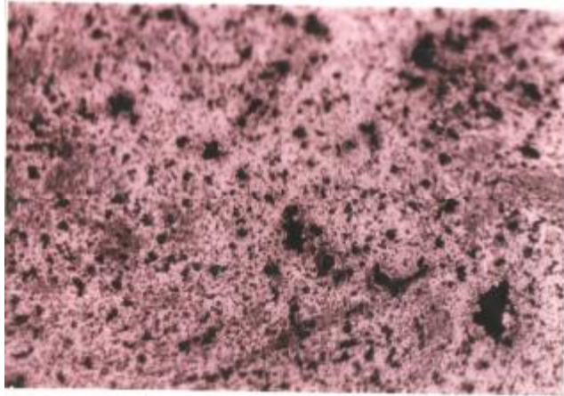
Figure (6) Microstructure of Fe-4% Cu alloys after water-quenched ((Massive Martensite with precipitates of Cu and some particles of Fe 2 O 3 or Cu 2 O)). (X200)
