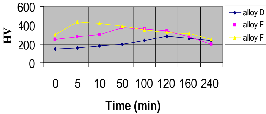
Figure (11 B ) Precipitation hardening of Fe-Cu-Ni alloy after water quenching and aging at 480 o C
