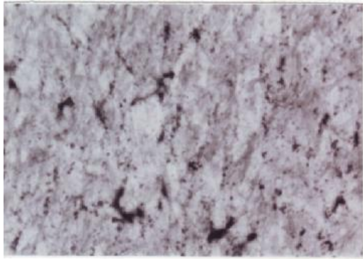
Figure (3) Microstructure of Fe-2% Cu alloys after air -cooled. ((Massive Ferrite with precipitates of Cu and some particles of Fe 2 O 3 or Cu 2 O)). (X200)
