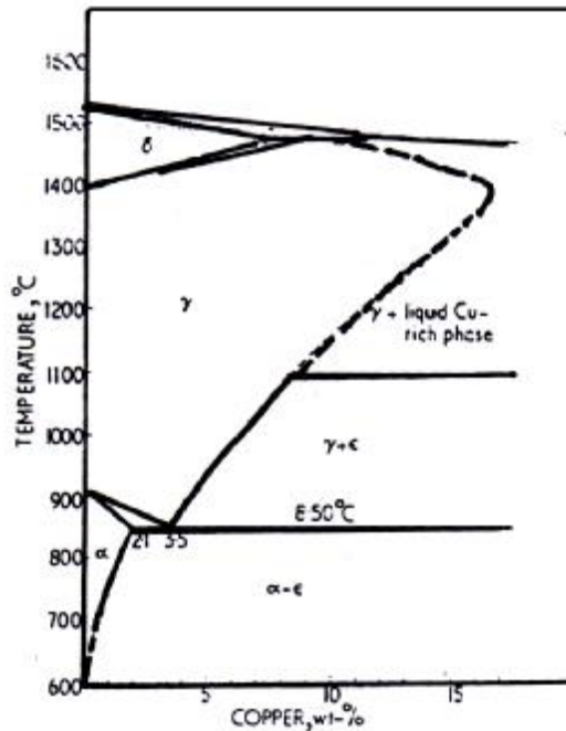
Figure (1) Iron rich end of the Fe-Cu diagram (1,2,3)
