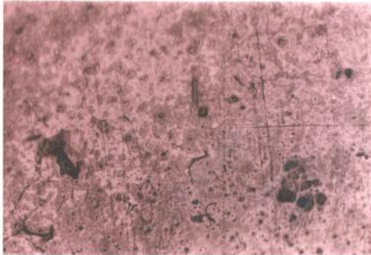
Figure (8) Microstructure of Fe-4% Cu-2%Ni alloys after air -cooled. (Massive Martensite with precipitates of Cu and some Particles of Fe 2 O 3 orCu 2 O orNi 2 O 3 )). (X200)
