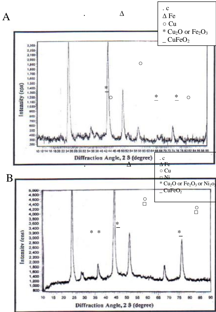
Figure (7) X- ray diffraction Analysis of alloys A-Fe-0.2%C-6%Cu B-Fe-0.2%C-6%Cu-3%Ni
