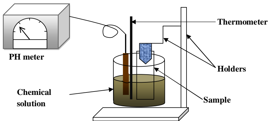
Figure (1) show the setup of deposition system
