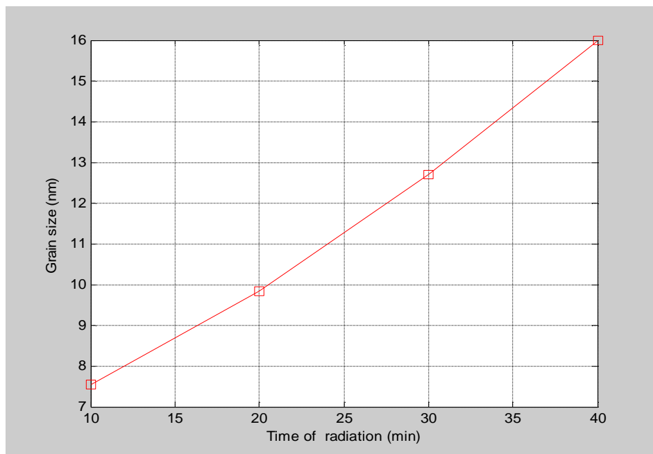
Figure (9) show the change in average of grain size in different time
