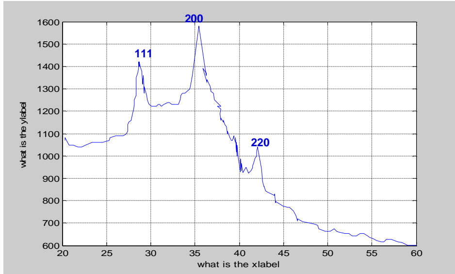
Figure (8) Show the crystalline structure of film after 40 min from irradiation
