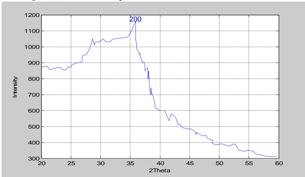
Figure (5) Show the crystalline structure of film after 10 min from irradiation
