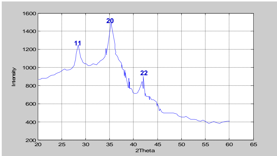
Figure (7) Show the crystalline structure of film after 10 min from irradiation
