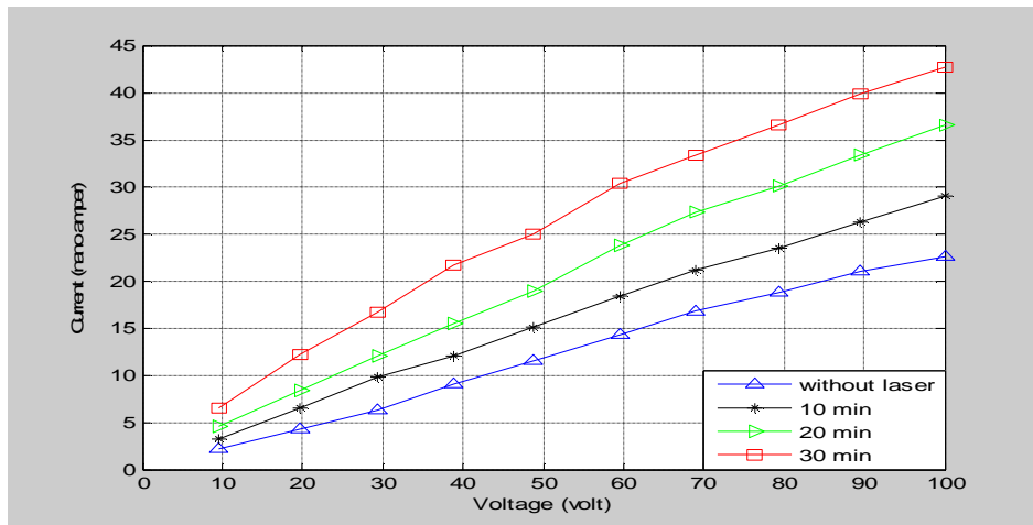
Figure (10) Show the change in electro conductivity before and after annealing
