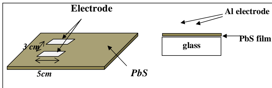
Figure (3) Show the shape of electrodes in the thin film
