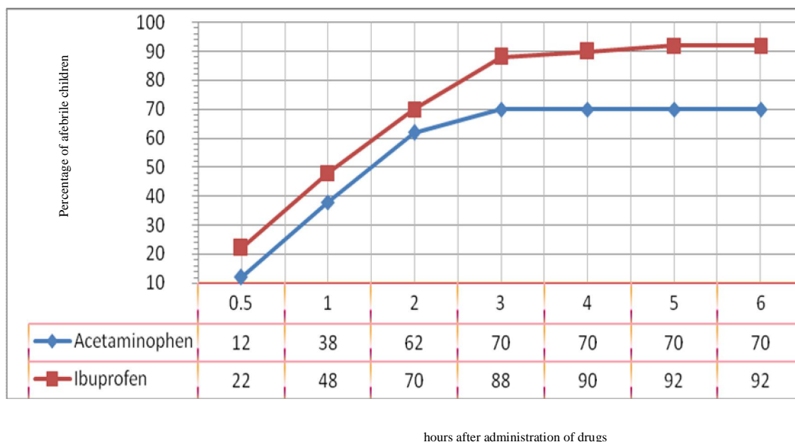
(Fig 1) . Percentage of afebrile patients during the following hours after administration of Acetaminophen and Ibuprofen.
