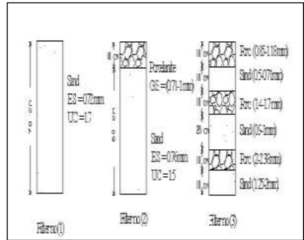
Fig.(3) Arrangement of layers of filter columns for set no. (2)
