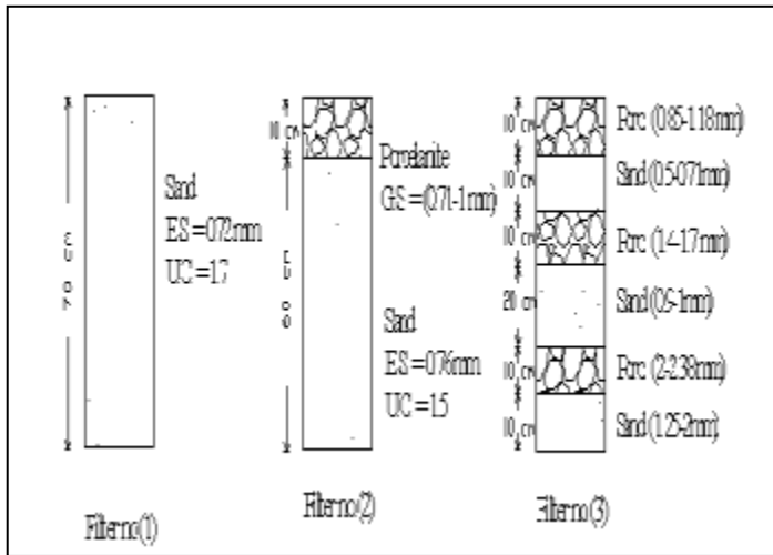
Fig.(2) Arrangement of layers of filter columns for set no. (1)
