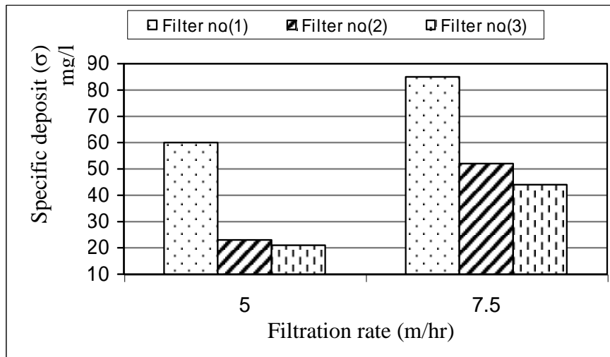
Fig (4) The average specific deposit for the three filters at different filtration rates in Set No. (1)
