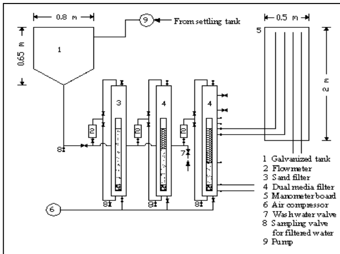
Fig.(1) Schematic diagram of the pilot filtration unit
