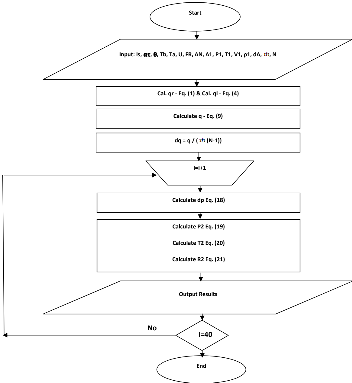
Figure (3) Program Flow Chart
