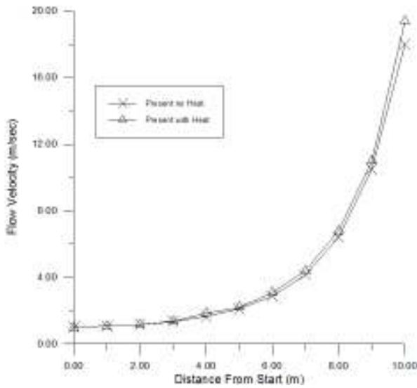
Figure(4)Variation of flow velocity along the nozzle
