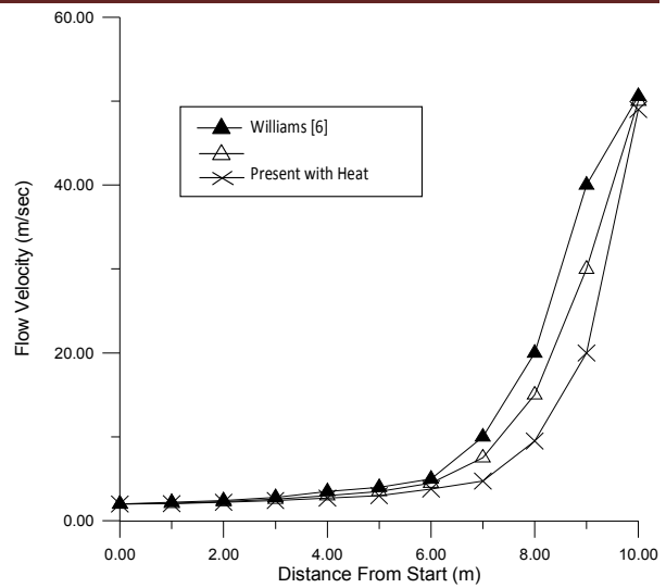
Figure (5) Comparison of flow velocity with, (Williams, 2007
