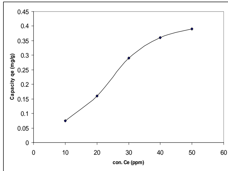
Fig. 5: Effect of initial concentration on the biosorption of metal ion onto sunflower shell biomass.
