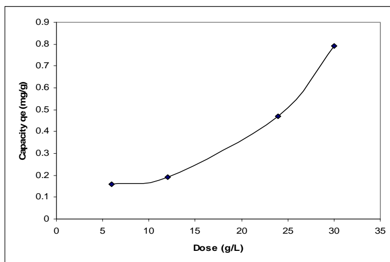
Fig. 7: Effect of dosage on the biosorption of metal ions onto sunflower shell biomass.
