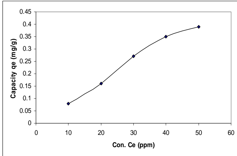
Fig. 4: Effect of initial concentration on the biosorption of metal ion onto wheat bran biomass.
