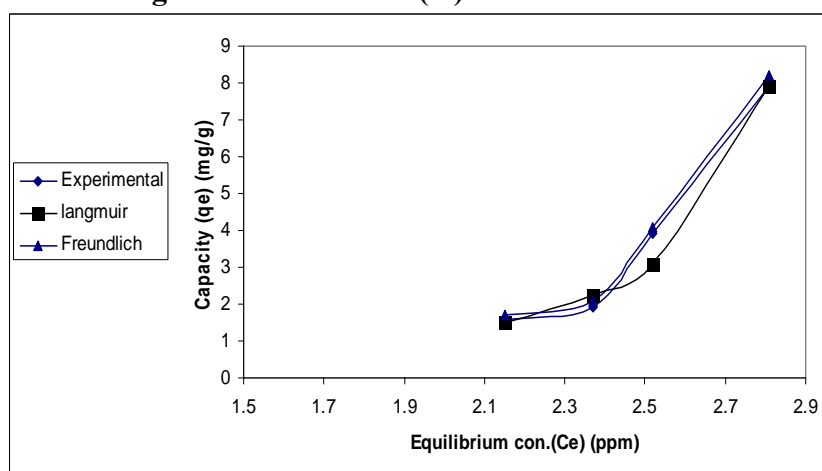
Fig 8: Isotherm of Cd(II) ion on wheat bran
