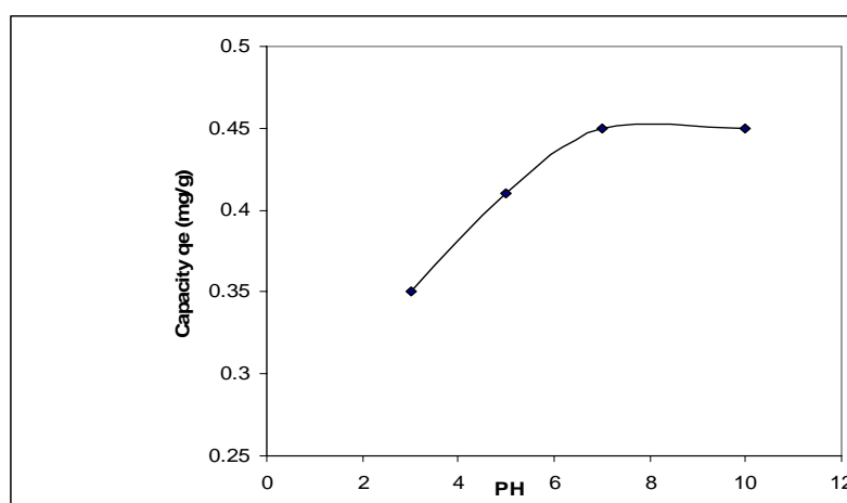
Fig. 2: Effect of pH on the biosorption of metal ion onto wheat bran biomass.
