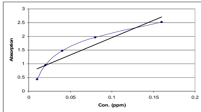
Fig.1: Calibration curve
