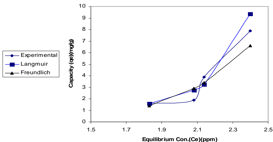
Fig 8: Isotherm of Cd(II) ion on wheat bran
