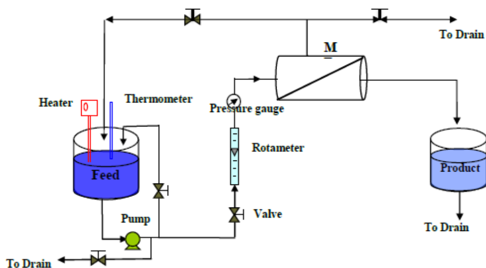
Fig. 2, Schematic Diagram of Microfiltration Process
