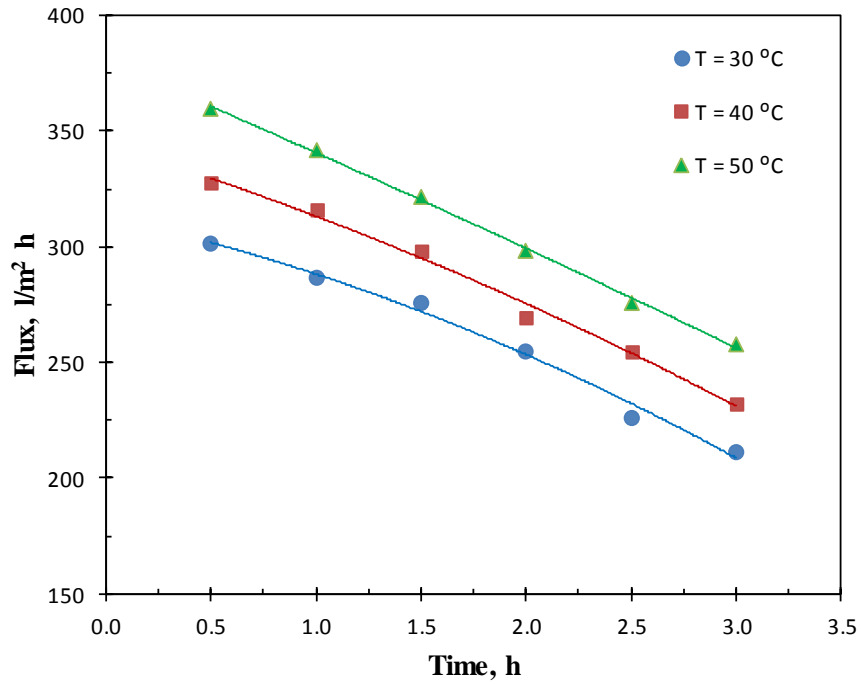
Fig. 7, Flux vs. Time at Different Feed Temperature (Ceramic 0.5 \mu\text{m} , Q_F = 25 l/h, Oil 20W-50 and C_F = 400 ppm)
