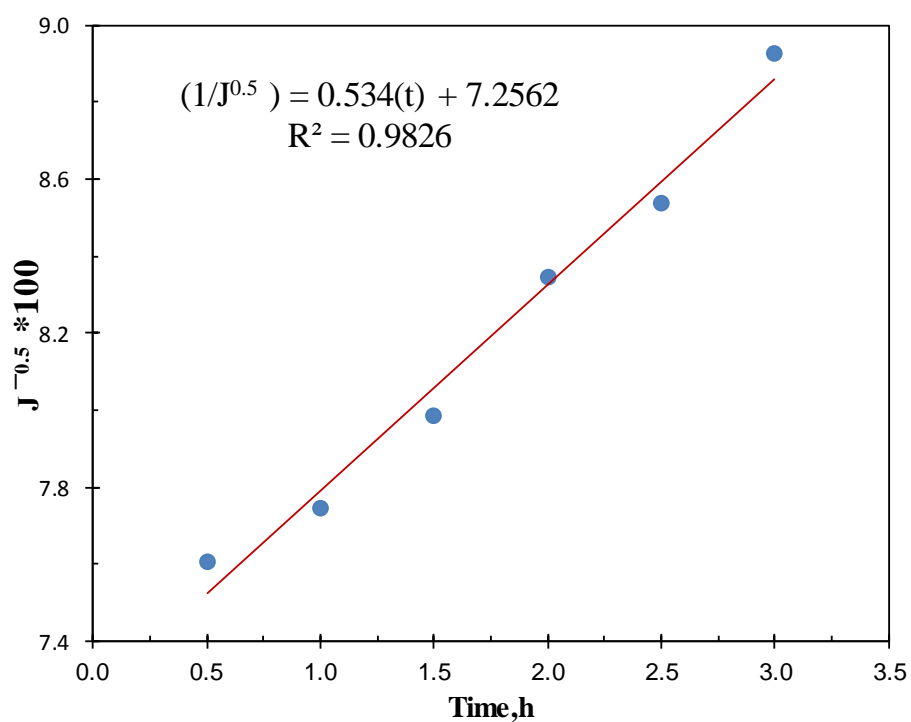
Fig. 14, Standard Pore Blocking Model ( C_F = 400 ppm, T = 30^\circ\text{C} and Q_F = 10 l/h)
