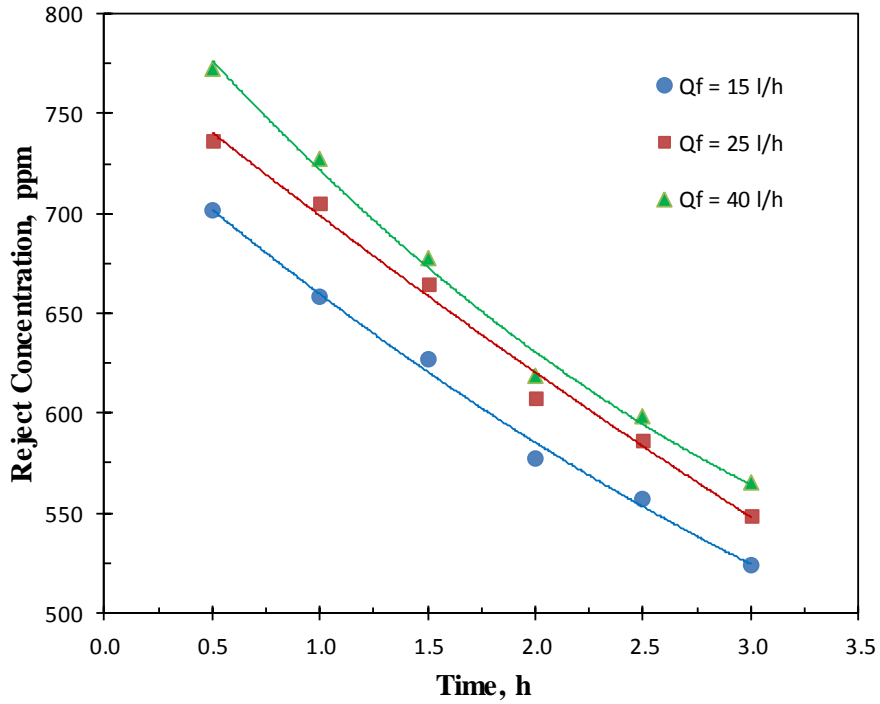
Fig. 12, Reject Concentration vs. Time at Different Feed Flow Rate (Ceramic 0.5 \mu m, C_F = 400 ppm, Oil 20W-50 and T = 40°C)
