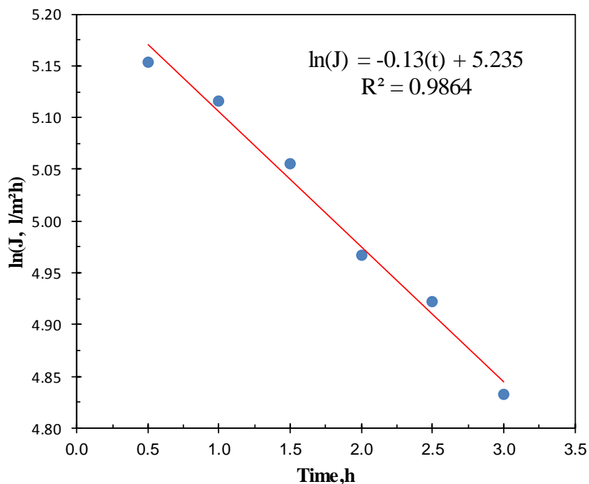
Fig. 13, Complete Pore Blocking Model ( C_F = 400 ppm, T = 30^\circ\text{C} and Q_F = 10 l/h)
