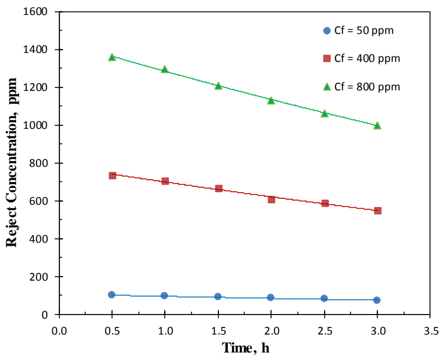
Fig. 6, Reject Concentration vs. Time at Different Oil Concentration (Ceramic 0.5 \mu m, Q_F = 25 l/h, Oil 20W-50 and T = 40^\circ\text{C} )
