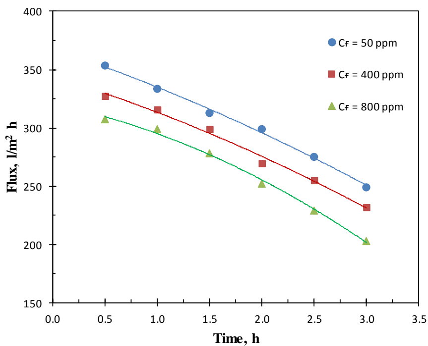
Fig. 4, Flux vs. Time at Different Oil Concentrations (Ceramic 0.5 \mu\text{m} , Q_F = 25 \text{ l/h} , Oil 20W-50 and T = 40^\circ\text{C} )
