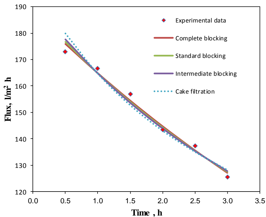
Fig. 17, Comparison of Filtration Model Prediction with Experimental Data for Polypropylene Membrane (1 \mu m)
