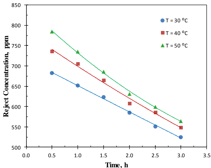
Fig. 9, Reject Concentrations vs. Time at Different Feed Temp. (Ceramic 0.5 \mu m, Q_F = 25 l/h, Oil 20W-50 and C_F = 400 ppm)
