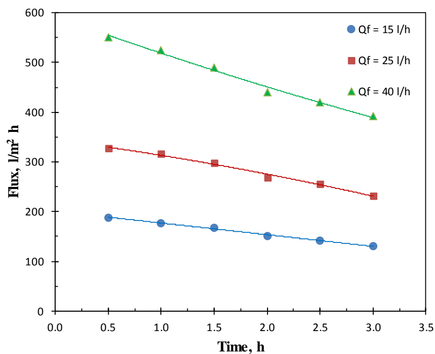
Fig. 10, Flux vs. Time at Different Feed Flow Rate (Ceramic 0.5 \mu m, T = 40^\circ\text{C} , Oil 20W-50 and C_F = 400 ppm)
