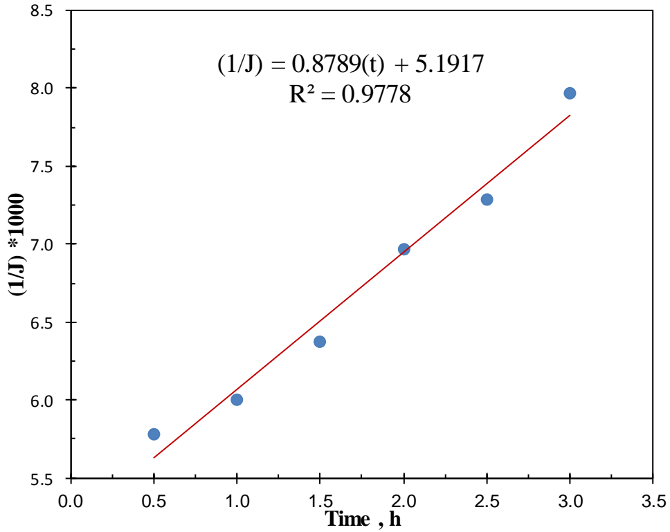
Fig. 15, Intermediate Pore Blocking Model ( C_F = 400 ppm, T = 30^\circ\text{C} and Q_F = 10 l/h)
