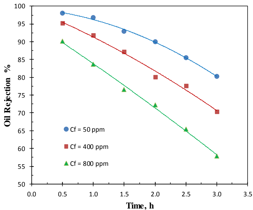
Fig. 5, Oil Rejection % vs. Time at Different Oil Concentrations (Ceramic 0.5 \mu m, Q_F = 25 l/h, Oil 20W-50 and T = 40^\circ\text{C} )
