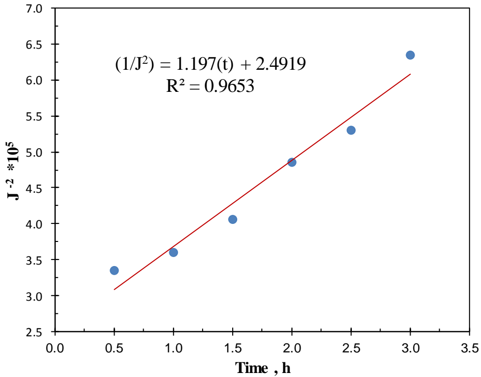
Fig. 16, Cake Filtration Model ( C_F = 400 ppm, T = 30^\circ\text{C} and Q_F = 10 l/h)
