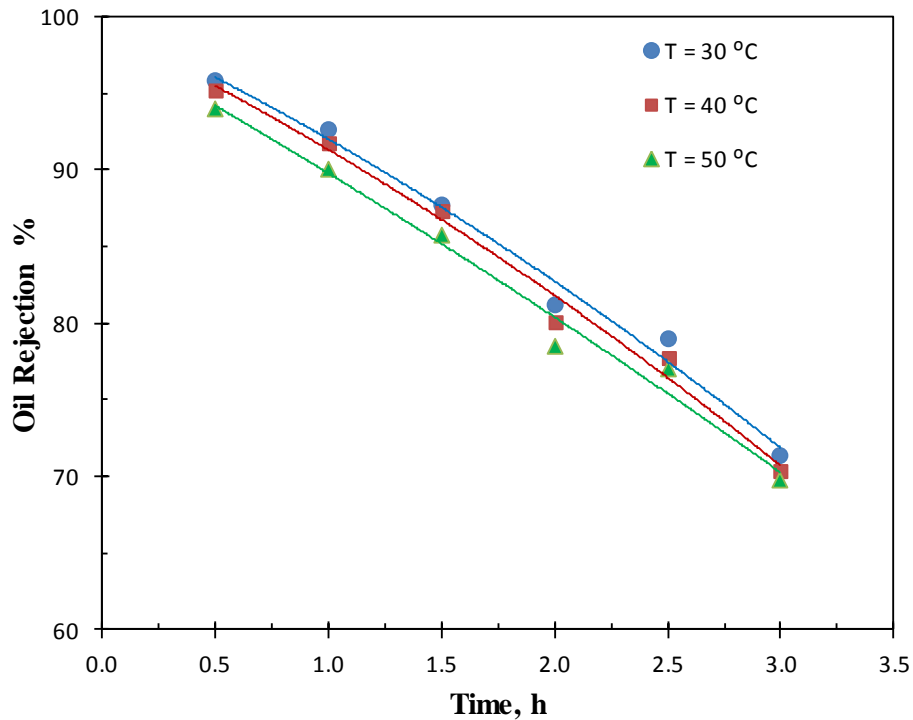
Fig. 8, Oil Rejection % vs. Time at Different Feed Temperature (Ceramic 0.5 \mu\text{m} , Q_F = 25 l/h, Oil 20W-50 and C_F = 400 ppm)
