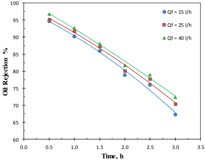
Fig. 11, Oil Rejection % vs. Time at Different Feed Flow Rate (Ceramic 0.5 \mu m, T = 40°C, Oil 20W-50 and C_F = 400 ppm)
