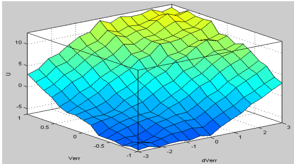
Figure (6) the control surface of the best designed FLC based exciter.
