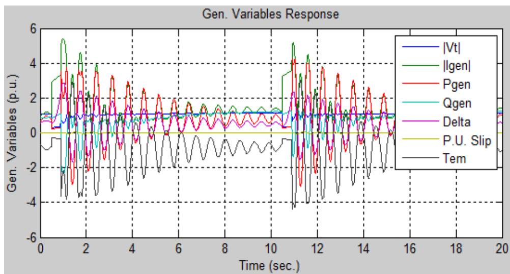
Figure (5) C Generator's variables response with the best FLC based exciter for 0.41 second clearing time.
