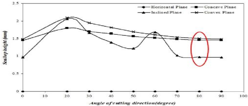
Figure (18). Best cutting direction angle for each plane using flat cutter.
