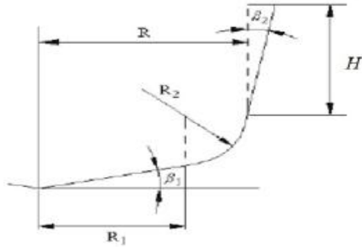
Figure (1) The definitions of a generalized cutter.[4]
