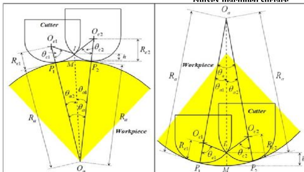
Figure.(4). Symbols of the mathematical model proposed
