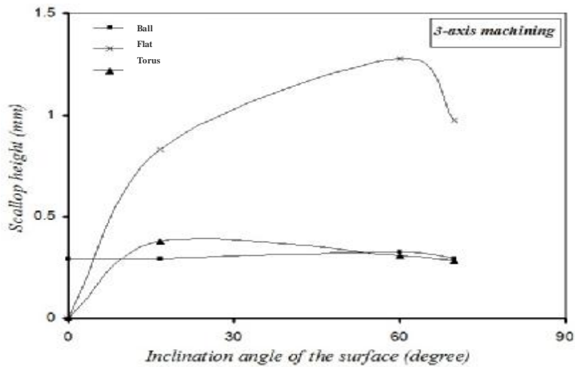
Figure (15) The effect of inclination angle of the surface on the value of scallop height using (ball, flat and torus) cutters on 3-axis machine.
