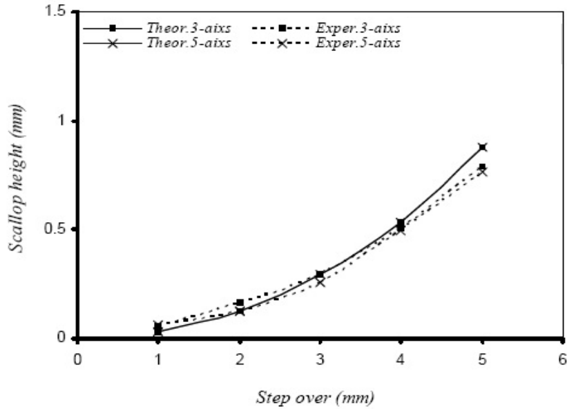
Figure.(14) Comparison between theoretical and experiment results.
