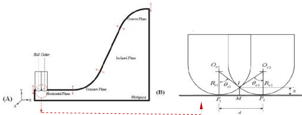
Figure.(5 A,B). Scallop height in horizontal plane by using ball cutter.
