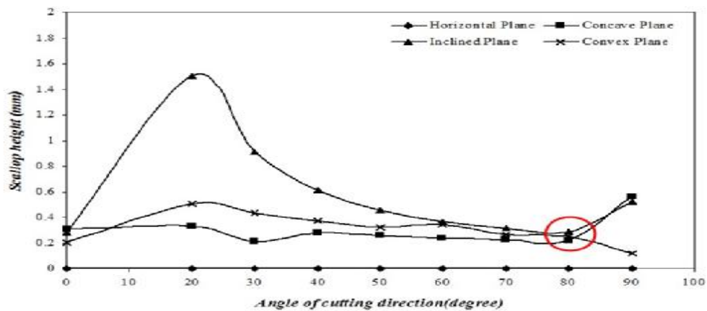
Figure.(19). Best cutting direction angle for each plane by using torus cutter.
