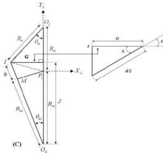
Figure (8 A, B and C). Scallop height in concave plane by using ball cutter for three and multi-axis machining.
