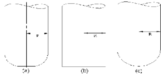
Figure (2) Different types of the end milling cutters. (a) torus cutter, (b) flat cutter, (c) ball cutter
