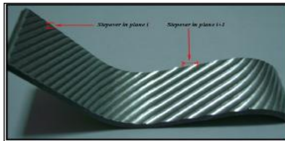
Figure (11) The magnitude of step over is change along the inclined plane when the angle of cutting direction 0^\circ \leq \alpha \leq 90^\circ .
