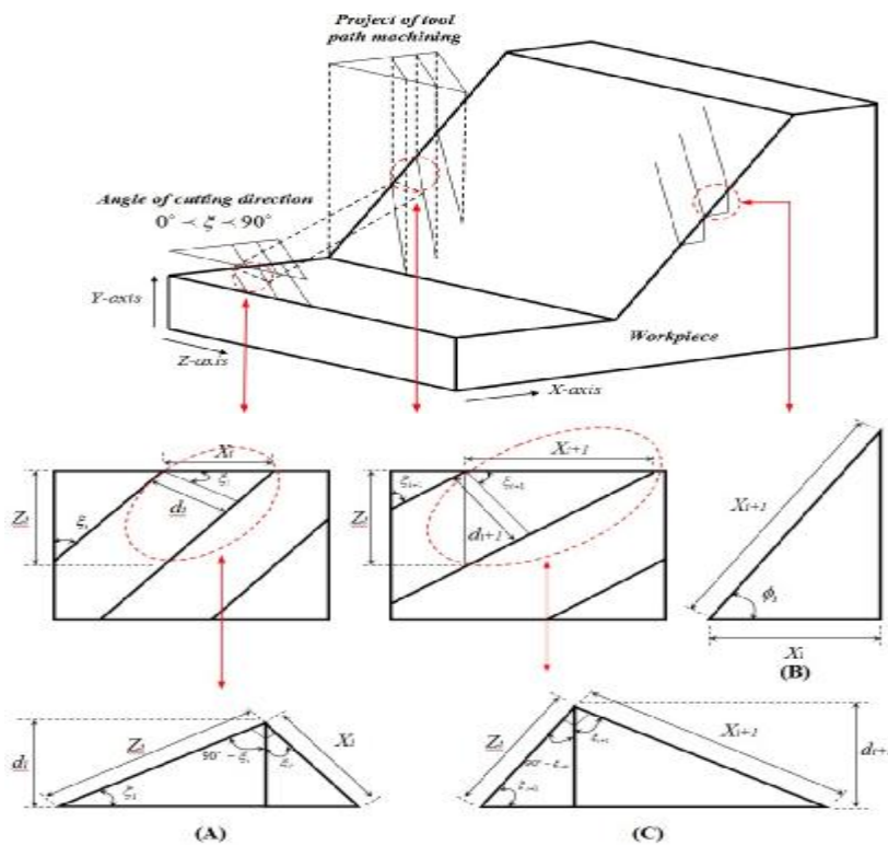
Figure (12 A,B and C) shows how step over is calculated in each plane if the angle of cutting direction 0^\circ \leq \alpha \leq 90^\circ : (A) explains step over in horizontal plane for (0^\circ \leq \alpha \leq 90^\circ) . (B) explains the geometrical shape to find X_{i+1} . (C) explains step over in inclined plane for (0^\circ \leq \alpha \leq 90^\circ) .
