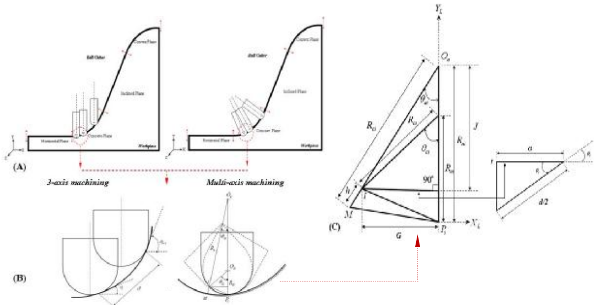
Figure (6 A,B and C). Scallop height in concave plane by using ball cutter for three and multi-axis machining.
