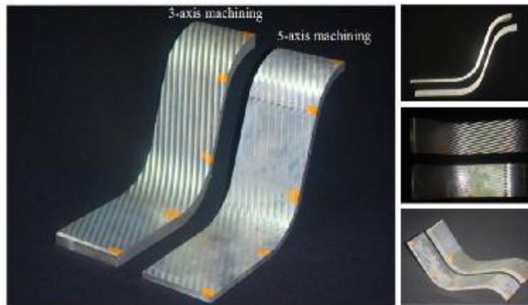
Figure.(13). The specimens after machining using 3 and 5-axis machine in CAD/CAM laboratory in Nanjing University in China.
