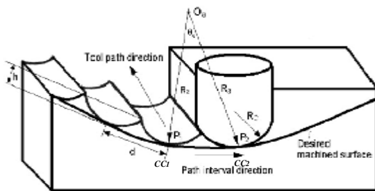
Figure (3a) Scallop heights for a concave machined surface.
