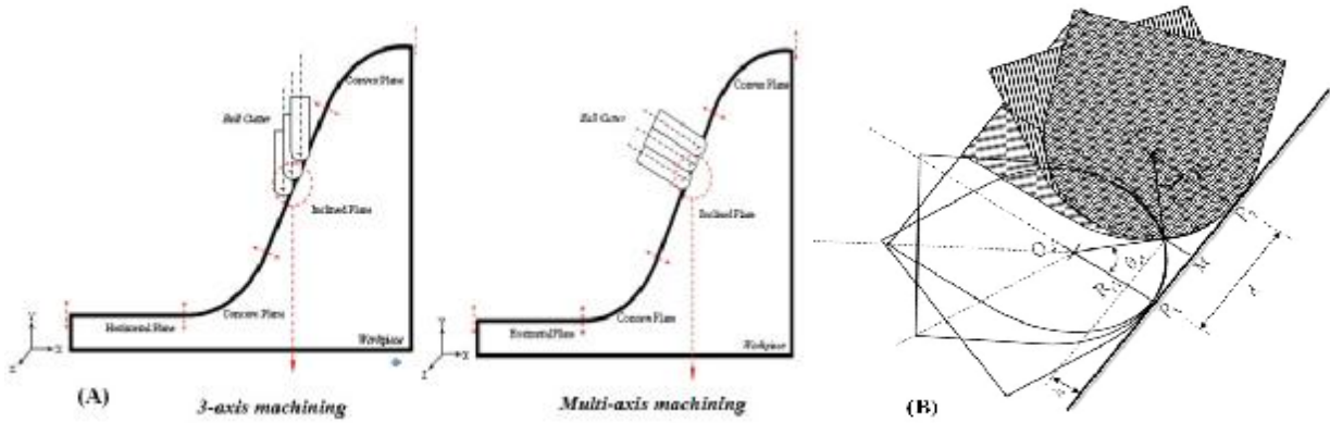
Figure.(7 A and B). Describes scallop height in inclined plane by using ball cutter for three and multi-axis machining.
