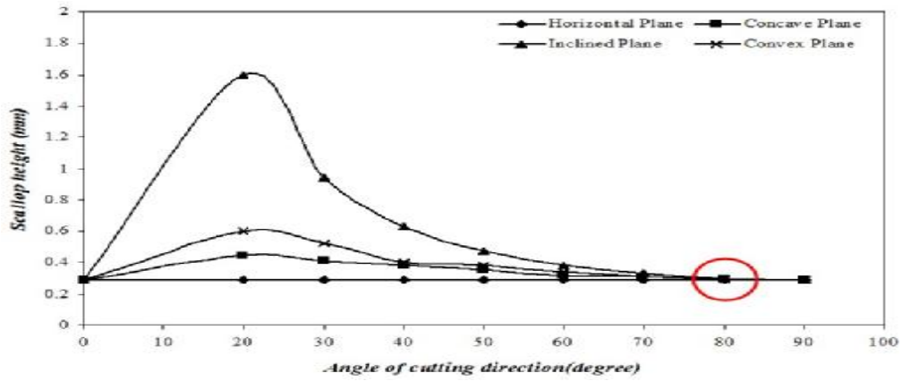
Figure (17) Best cutting direction angle for each plane using ball cutter.
