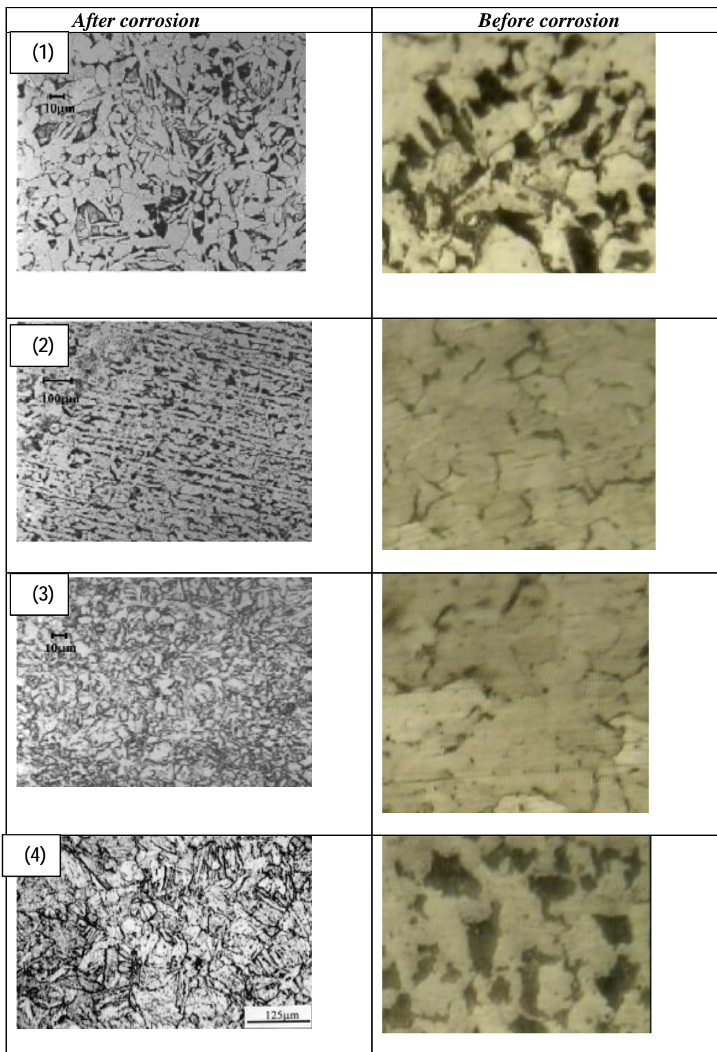
Figure 4: Photographs taken of the various microstructures of carbon steel:
