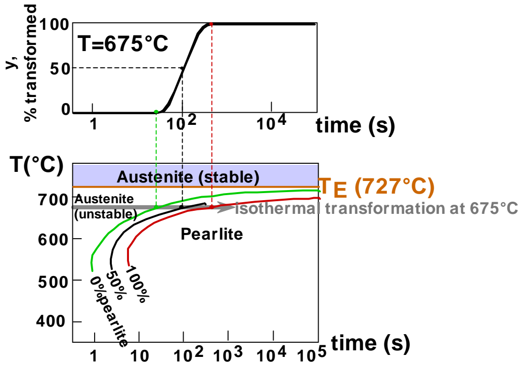
(B) Rapidly cool to 675 °C and hold isothermally
