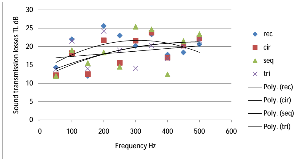
Figure (20): the trend polynomial second order values of figure (14).
