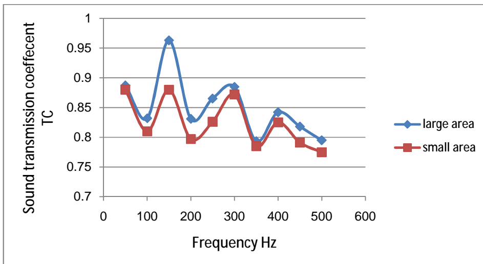
Figure (17):TC for Triangular orifice case
