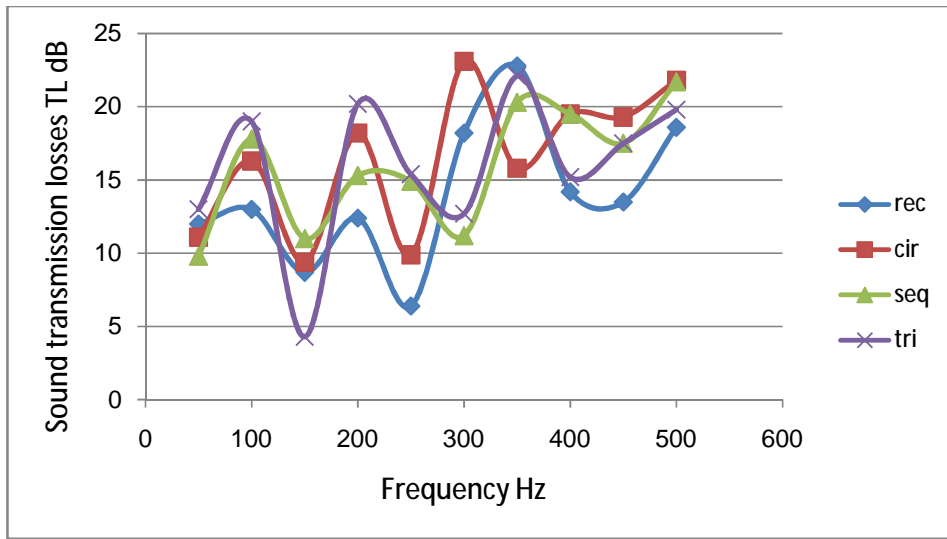
Figure (12): comparison for TL values between the four models with large area
