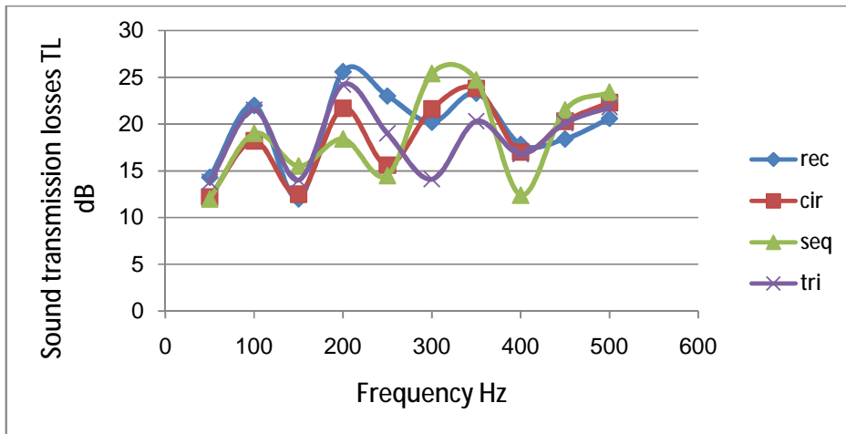
Figure (13):comparison for TL values between the four models with small area
