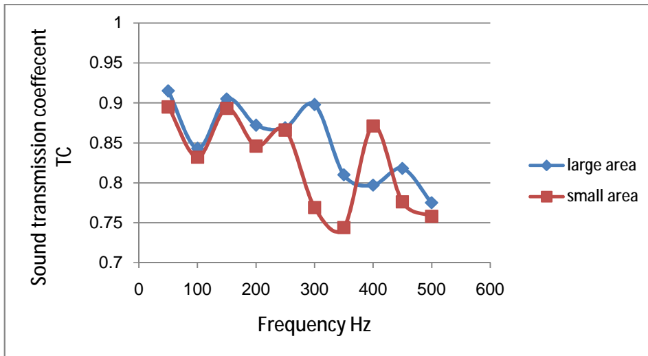
Figure (16):TC for Square orifice case
