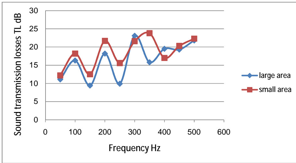
Figure (8): TL for Circular orifice case
