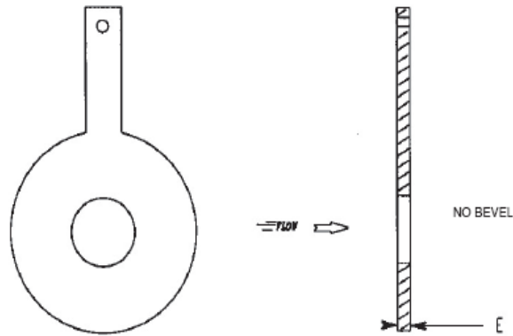
Figure (1)Restriction Orifice plate
