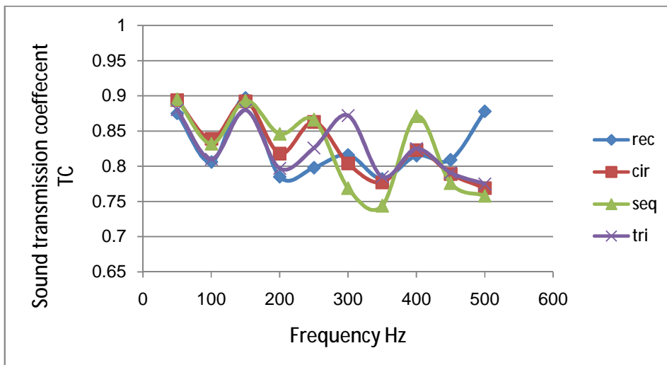
Figure (19):comparison for TC values between the four models with small area
