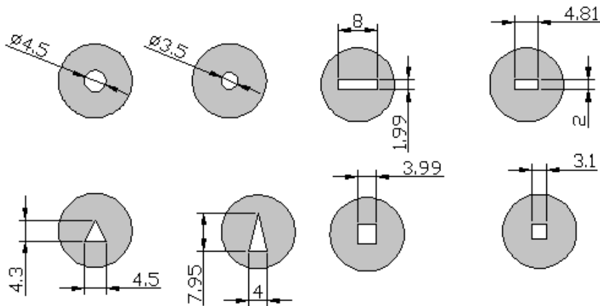
Figure (7): a schematic for the orifice plate samples
