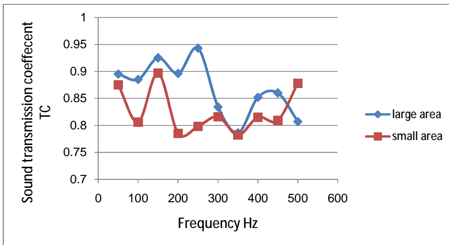
Figure(15):TC for Rectangular orifice case
