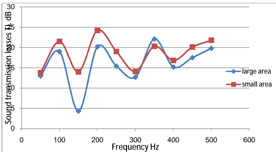
Figure (11): TL for Triangular orifice case
