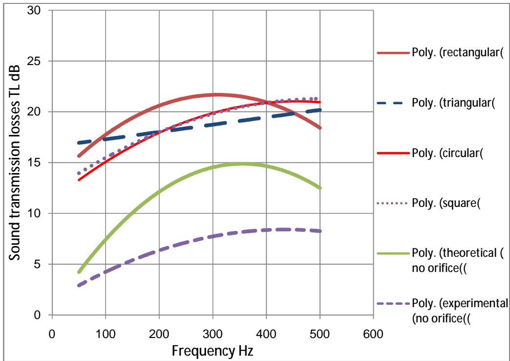
Figure (22):A comparison for the theoretical values of (TL with no orifice) and the experimental values with and without orifice.
