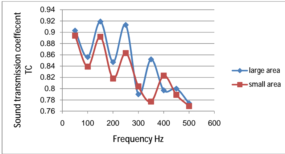
Figure (14):TC for Circular orifice case
