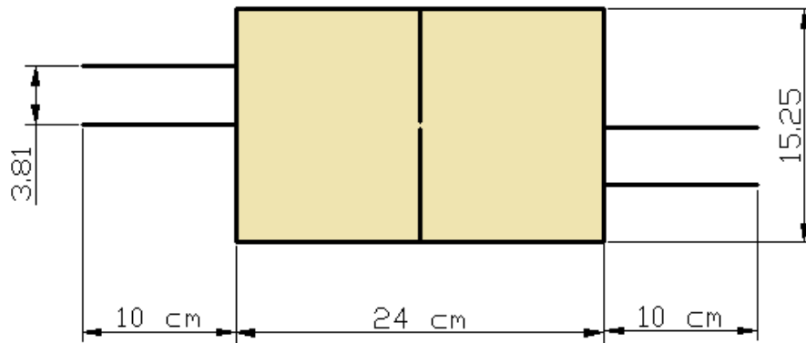
Figure (1)Restriction Orifice plate
