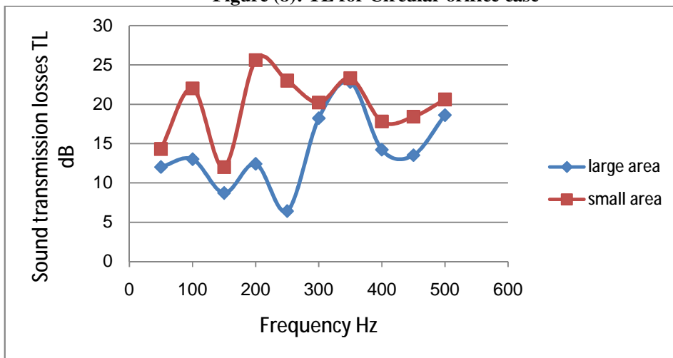
Figure (9): TL for Rectangular orifice case
