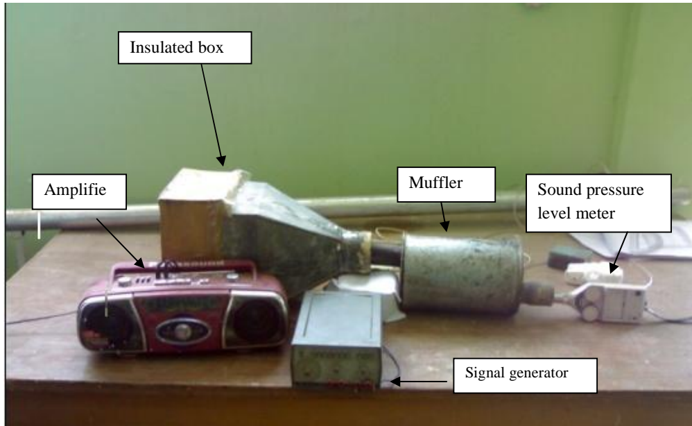
Figure (4) the test parts photo.
