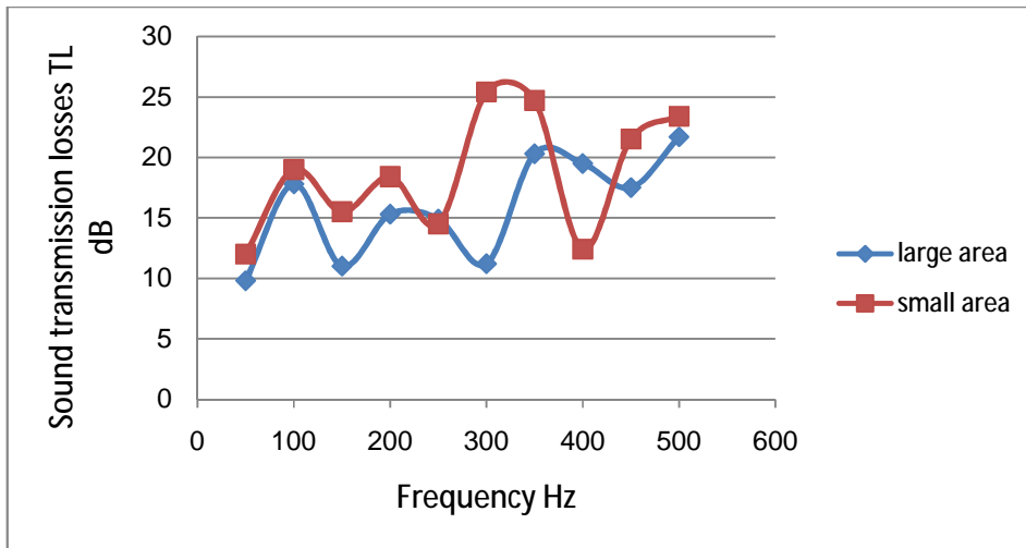
Figure (10): TL for Square orifice case
