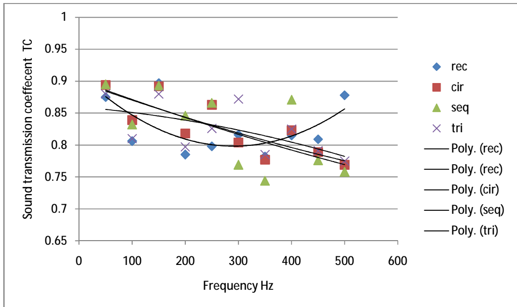
Figure(21): The trend polynomial second order values of figure (20).
