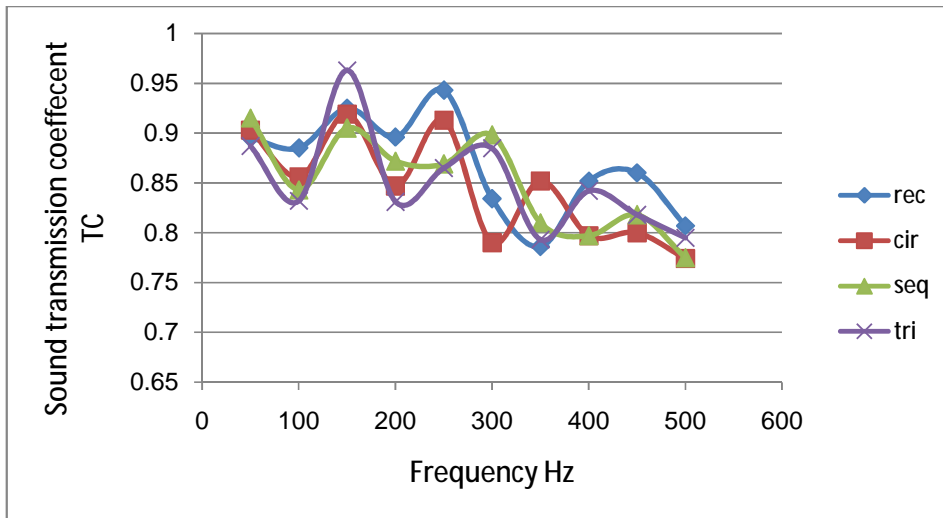
Figure(18):comparison for TC values between the four models with large area
