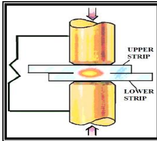
Figure (1) shows the RSW process.
