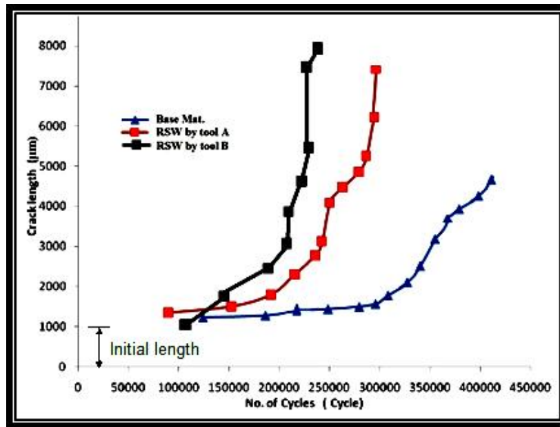
Figure (7) Relationship between crack length and cycles.
