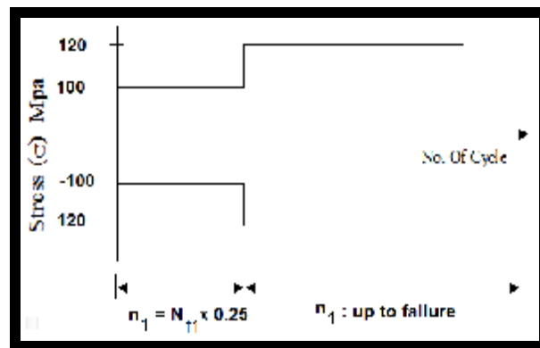
Figure (5) shows Variable fatigue loading.
