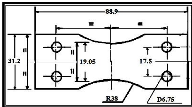
Figure (3) shows drawing detail of specimen.
