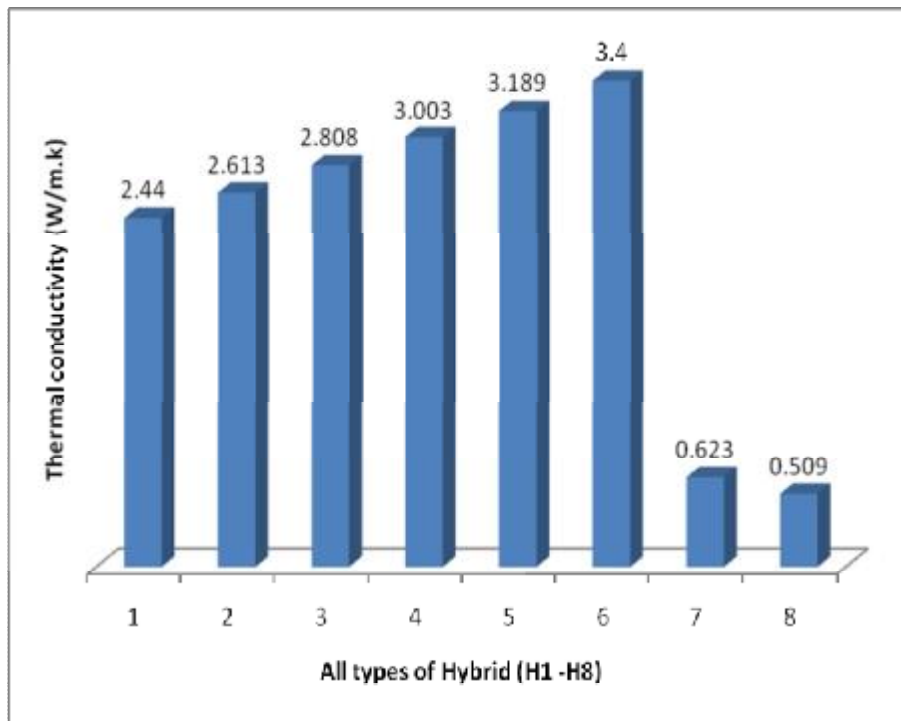
Figure (8) Experimental thermal conductivity for parallel arrangement
