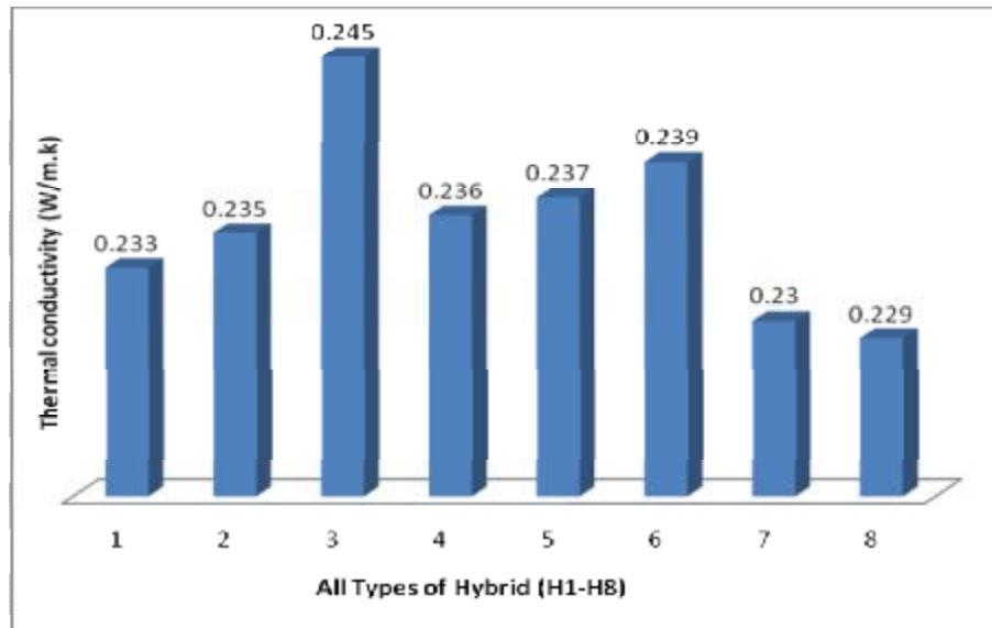
Figure (9) Experimental thermal conductivity for perpendicular arrangement
