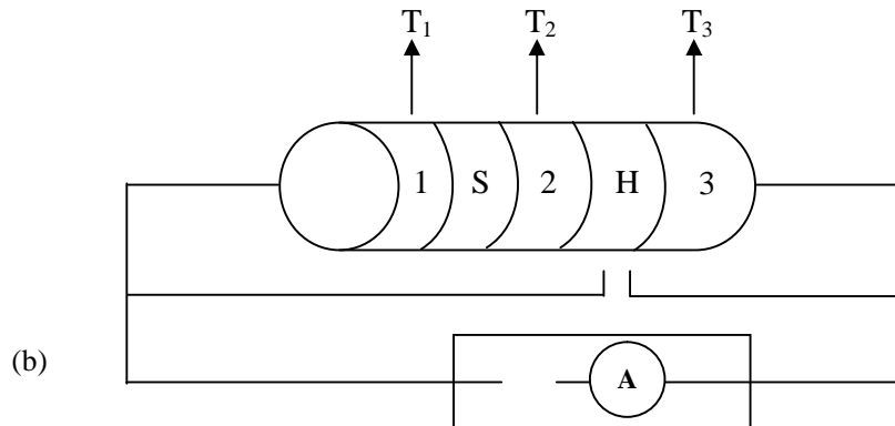
Figure (2) (a) shows the instrument of the thermal conductivity (b) the distribution of ( T_1, T_2, T_3 ).
