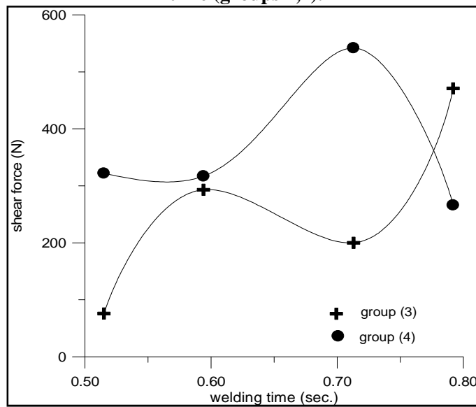
Figure (9) variation of shear force with the welding Time (groups3, 4).
