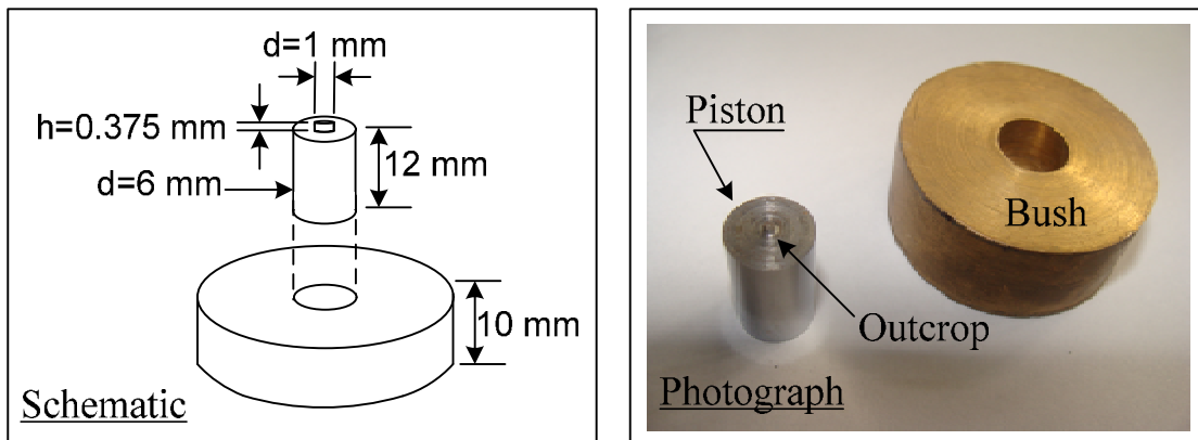
Figure (5) schematic and photography of gap die.
