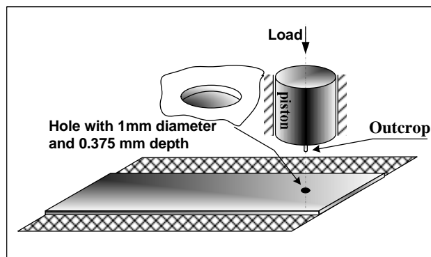
Figure(6) schematic diagram of making gap mechanism.
