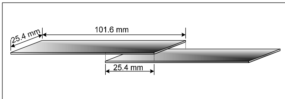
Figure (2) overlapping the two pieces of spot welding specimen.
