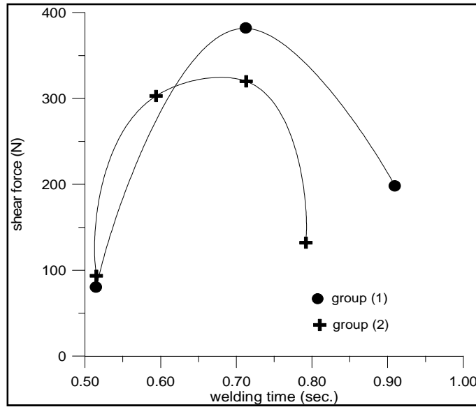
Figure (8) variation of shear force with the welding time (groups 1,2).
