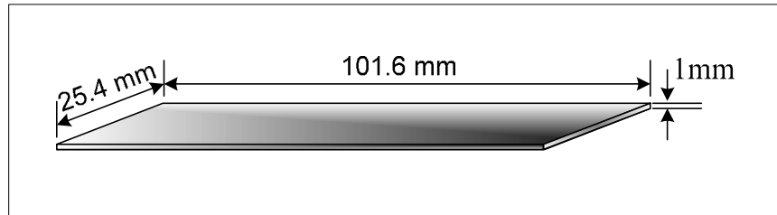
Figure (1) standard spot welding piece.
