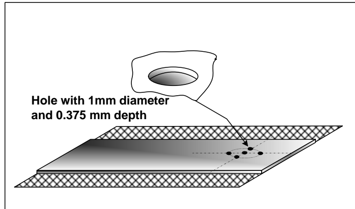
Figure (11) schematic diagram of gap arrangement.
