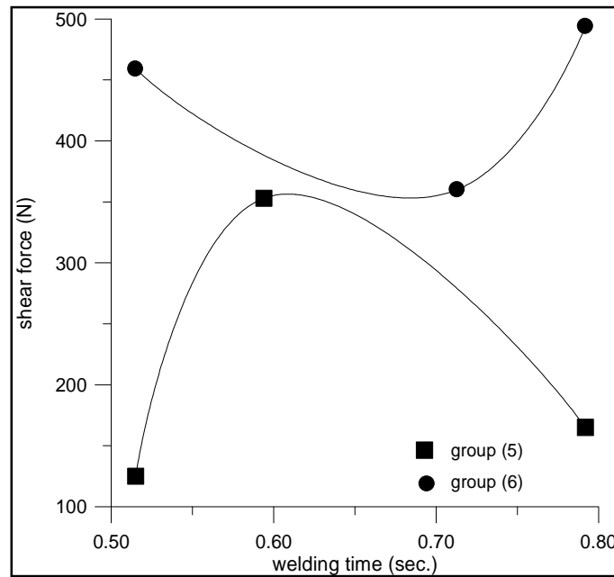
Figure (10) variation of shear force with the welding time (groups 5,6).
