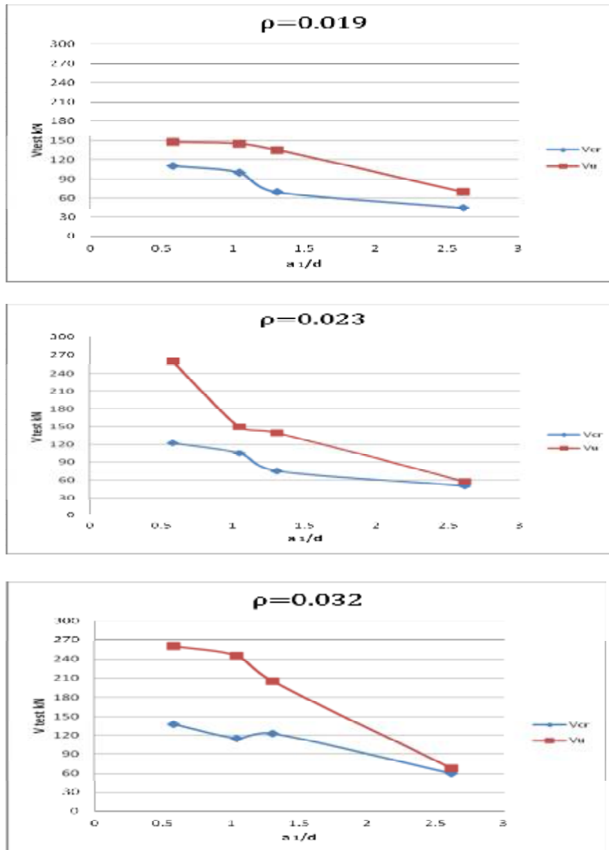
Figure (3) Effect a_1/d Ratio on Shear Strength of RC Beams.
