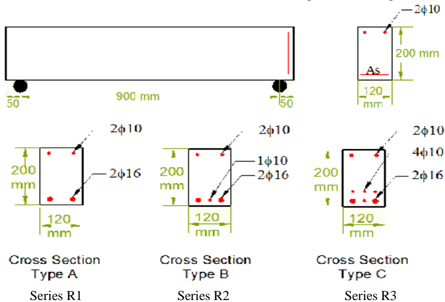
Figure (1) Beam Reinforcement Details.
