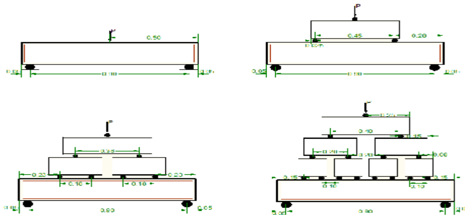
Figure (2) 1, 2, 4, 8 Point Loads.
