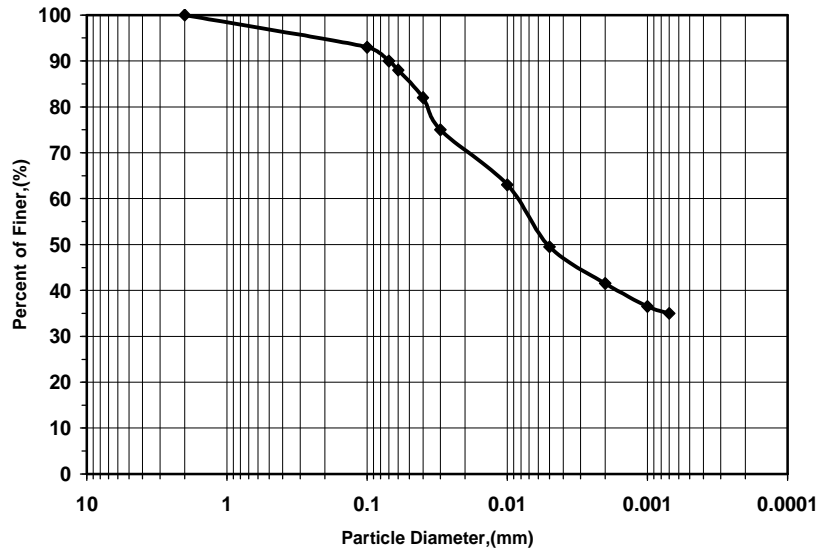
Figure (1). Grain Size Distribution of Soil Used
