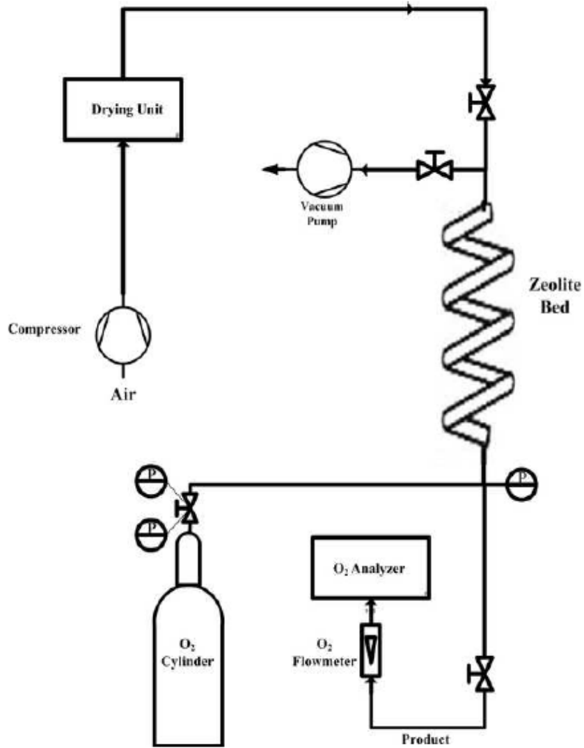
Figure (3) Experimental setup.
