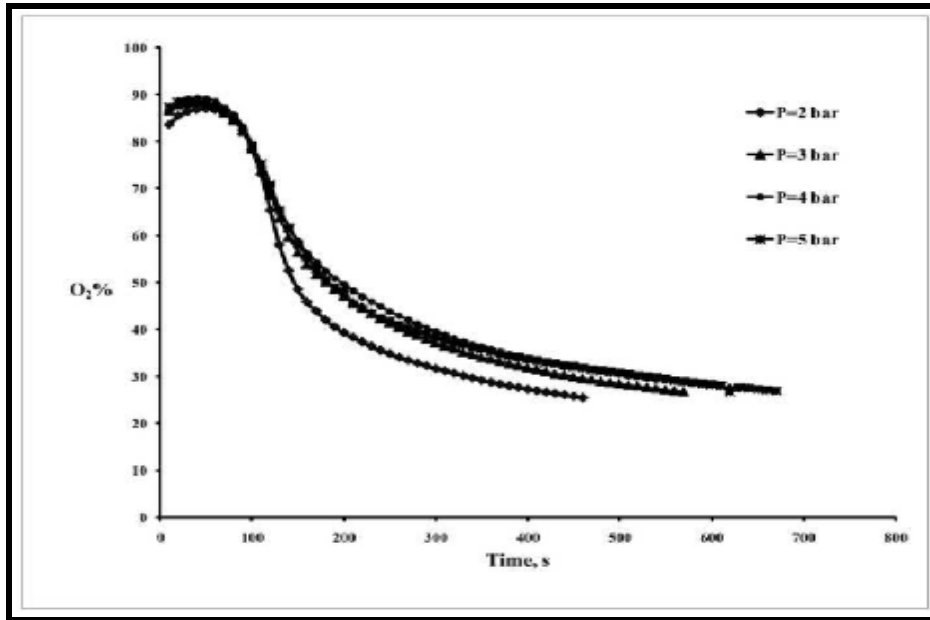
Figure (4) Breakthrough curve, using air feed pressurizing at different adsorption pressures and Q_{\text{eff}}=1 lit/min.
