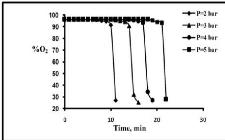
Figure (5) Breakthrough curve, by intermediate initial pure oxygen Pressurizing at Q_{\text{eff}}= 1 lit/min.
