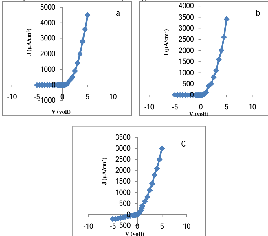
Figure (3) Dark, forward bias and reverse bias I –V characteristics of PS 15 mA/cm 2 at etching time 10 (b) 30 (c) 45 min.
