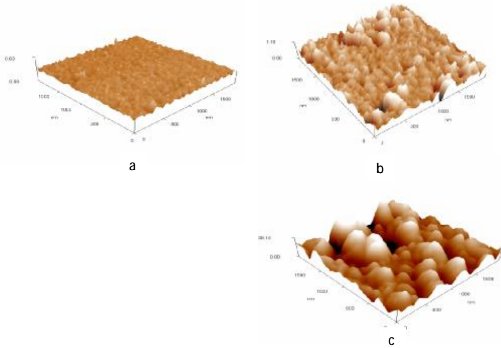
Figure (2) 3D AFM image of porous silicon prepared at J=15 mA/cm 2 etched under different etching time (a) 10, (b) 30 and (c) 45 min.
