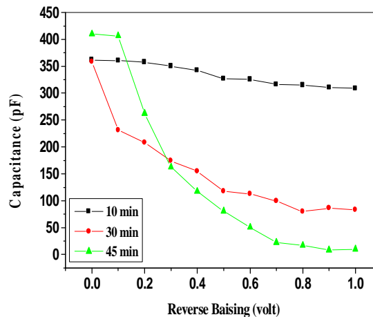
Figure (4): The Capacitance -Voltage characteristics for different etching Times 10, 30 & 45 min, and current density 15 \text{ mA/cm}^2 .
