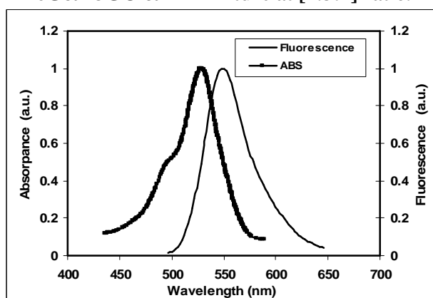
Figure (9) Absorption and fluorescence spectrum of R 6G&R3GO & RB mixture at [1:4:1] ratio.
