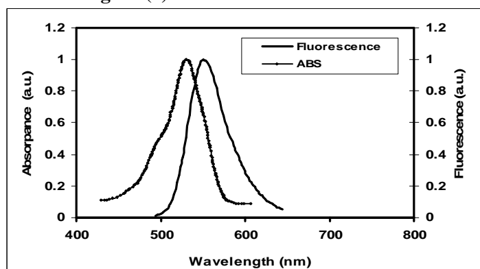
Figure (3) Absorption and Fluorescence Spectrum of R.
