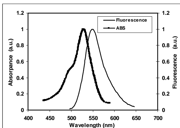
Figure (8) Absorption and fluorescence spectrum of R 6G&R3GO &R B mixture at [1:3:1] ratio.
