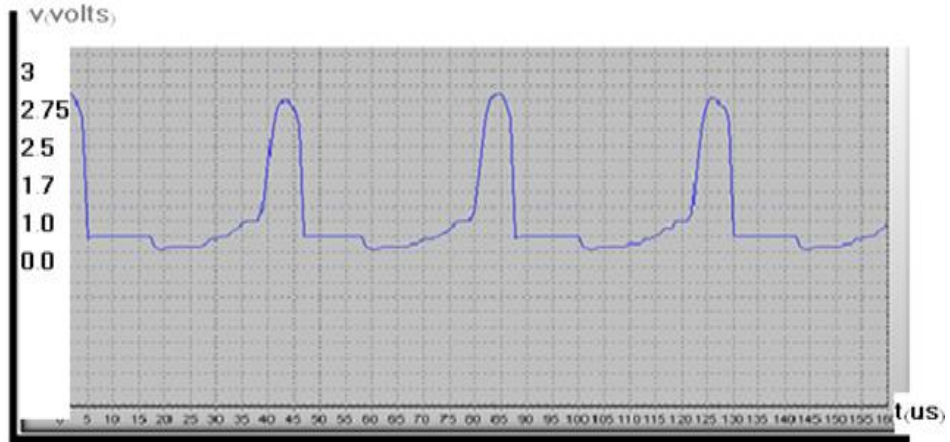
Figure (15a) O/p of pulse transformer to thyristor.
