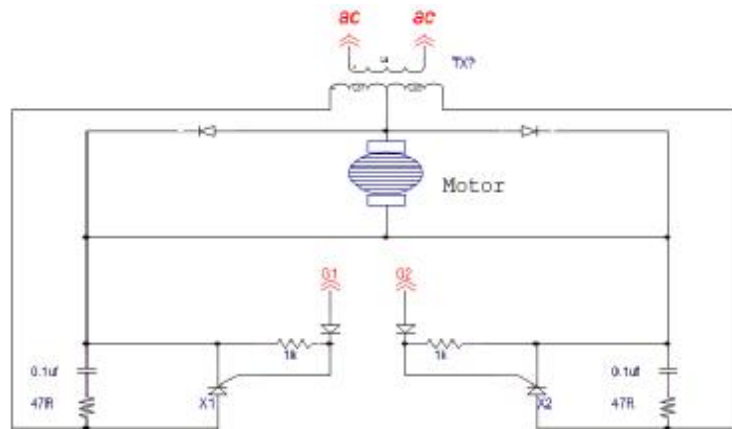
Figure (13) Power thyristor section.
