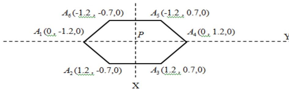
Figure (5) coordinates of moving platform.
