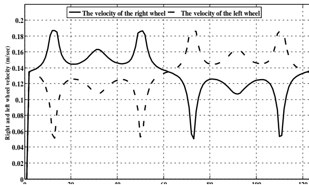
Figure (5) the right and left wheel action.
