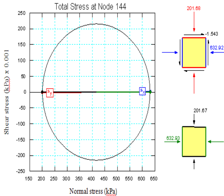
Figure (12b) Mohr circle on the node 144 at the invert after tunnel excavation.
